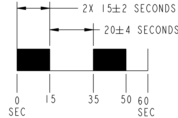
TIMER SWITCH No. 13-SPRAY (REF. ONLY)
