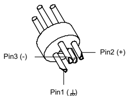
XLR, symmetric
