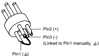
XLR, asymmetric
