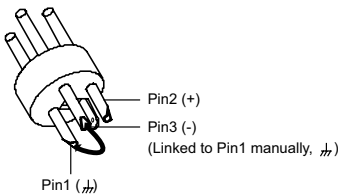
XLR, asymmetric
