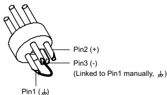
XLR, asymmetric
