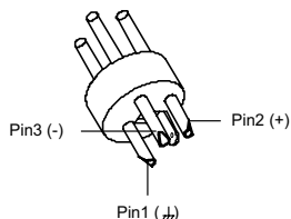
XLR, symmetric
