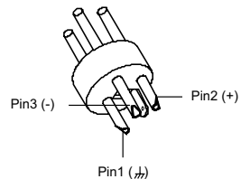
XLR, symmetric
