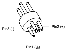
XLR, symmetric
