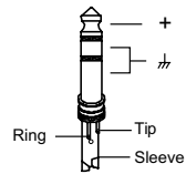
Stereocinch, asymmetric
