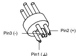
XLR, symmetric
