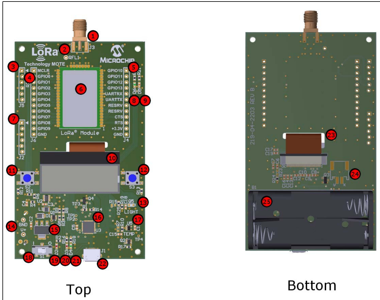
FIGURE 1-1: LoRa ® MOTE
