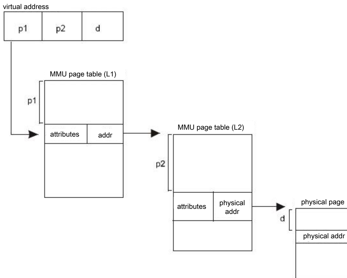
Figure 3-2. Virtual and Physical Addresses
