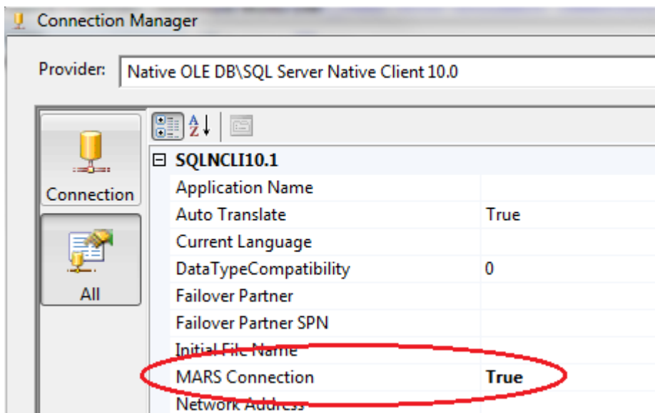
Figure 77 - Setting MARS in a DSV
