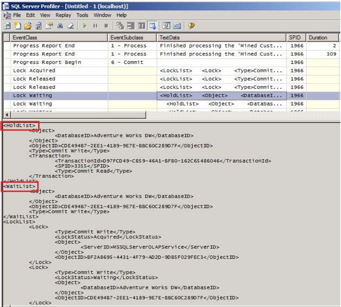
Figure 31 – SQL Server Profiler output of lock events
