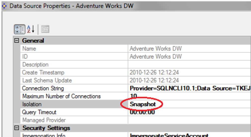
Figure 76 - Setting the Data Source to Snapshot
