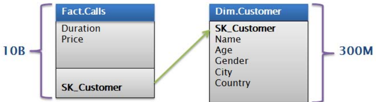
Figure 88: Call detail records (CDRs)
