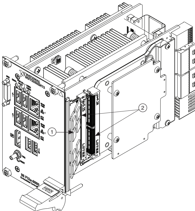
Figure 4-2. Installing a DDR4 SO-DIMM in an NI PXIe-8880 Controller
