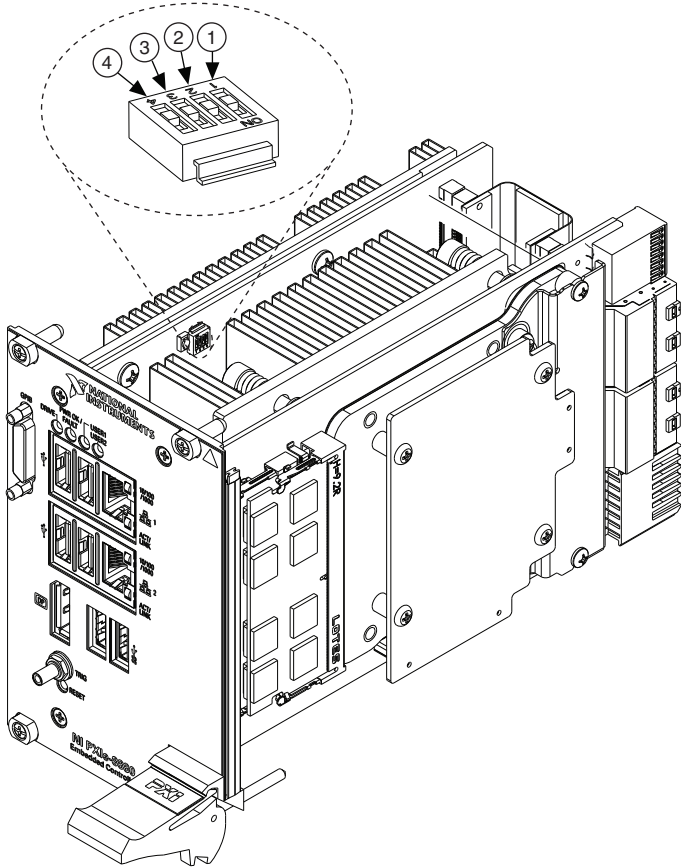
Figure 2-4. LabVIEW RT Configuration Switches
