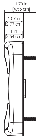
P40N+ Side Dimensions
