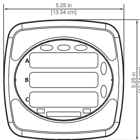
P40N+ Front Dimensions
