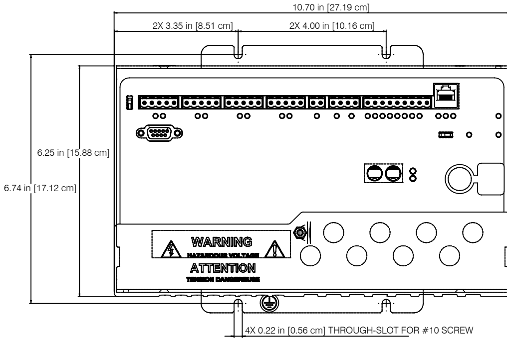
Nexus® 1450 Meter Front Dimensions
