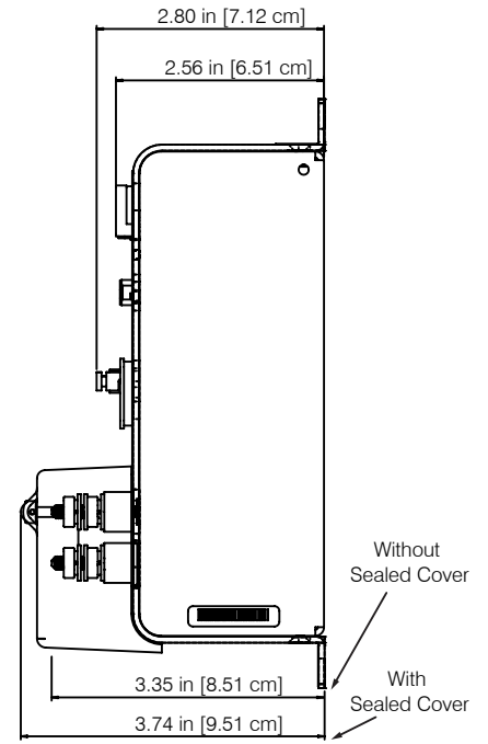
Nexus® 1450 Meter Side Dimensions
