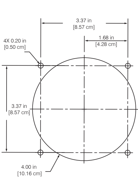
P40N+ Back Dimensions
