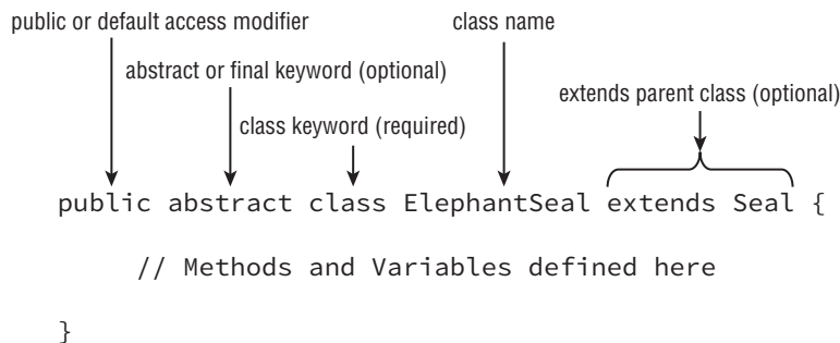
FIGURE 5.2 Defining and extending a class
