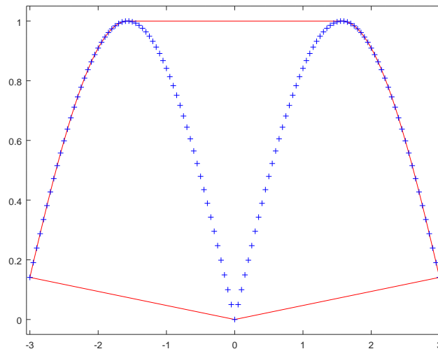
Figure 30.5: The convex hull of a simple set of points
