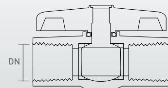
PVC roscar
