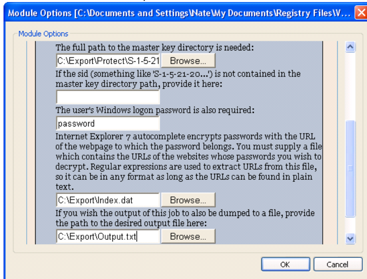
FIGURE 9-5 Module Options.
