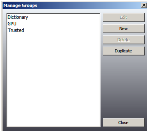
FIGURE 4-9 Manage Groups.
