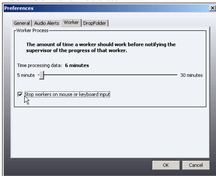
FIGURE 5-8 Worker Preferences
