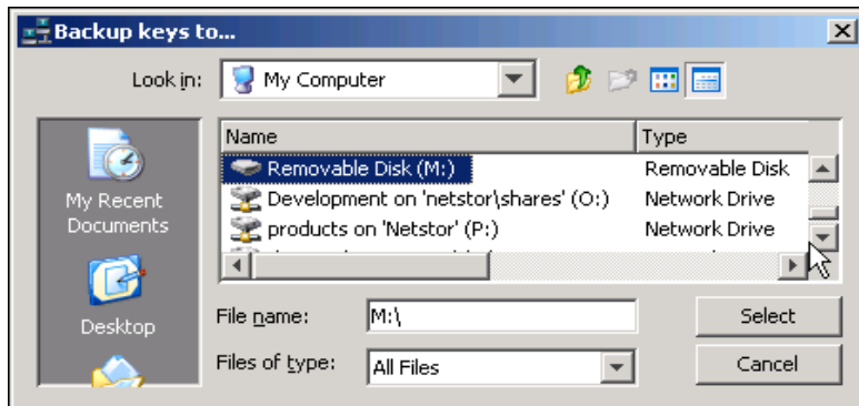
FIGURE 4-3 Backup Keys
