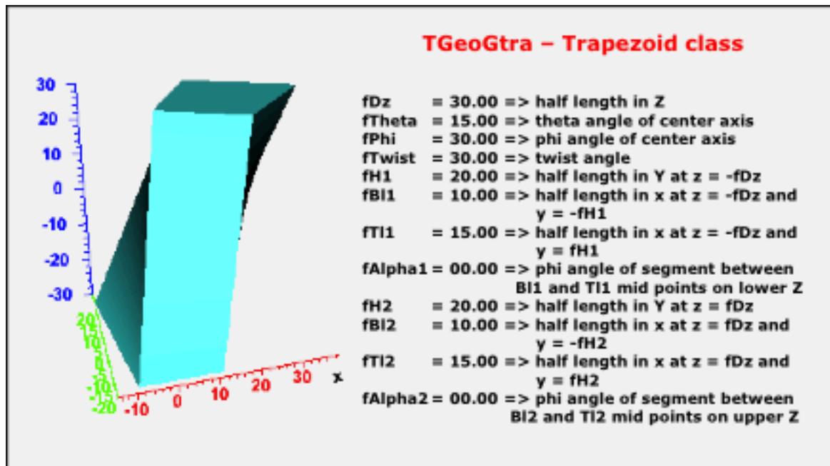
Figure 18.9: TGeoGtra class
