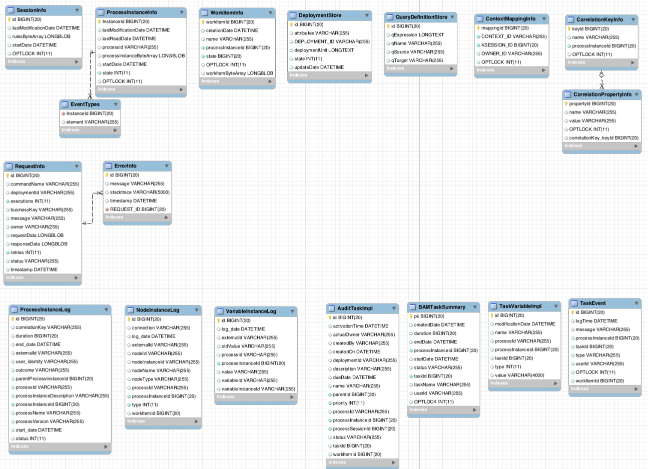
Figure 13.1. Data Model
