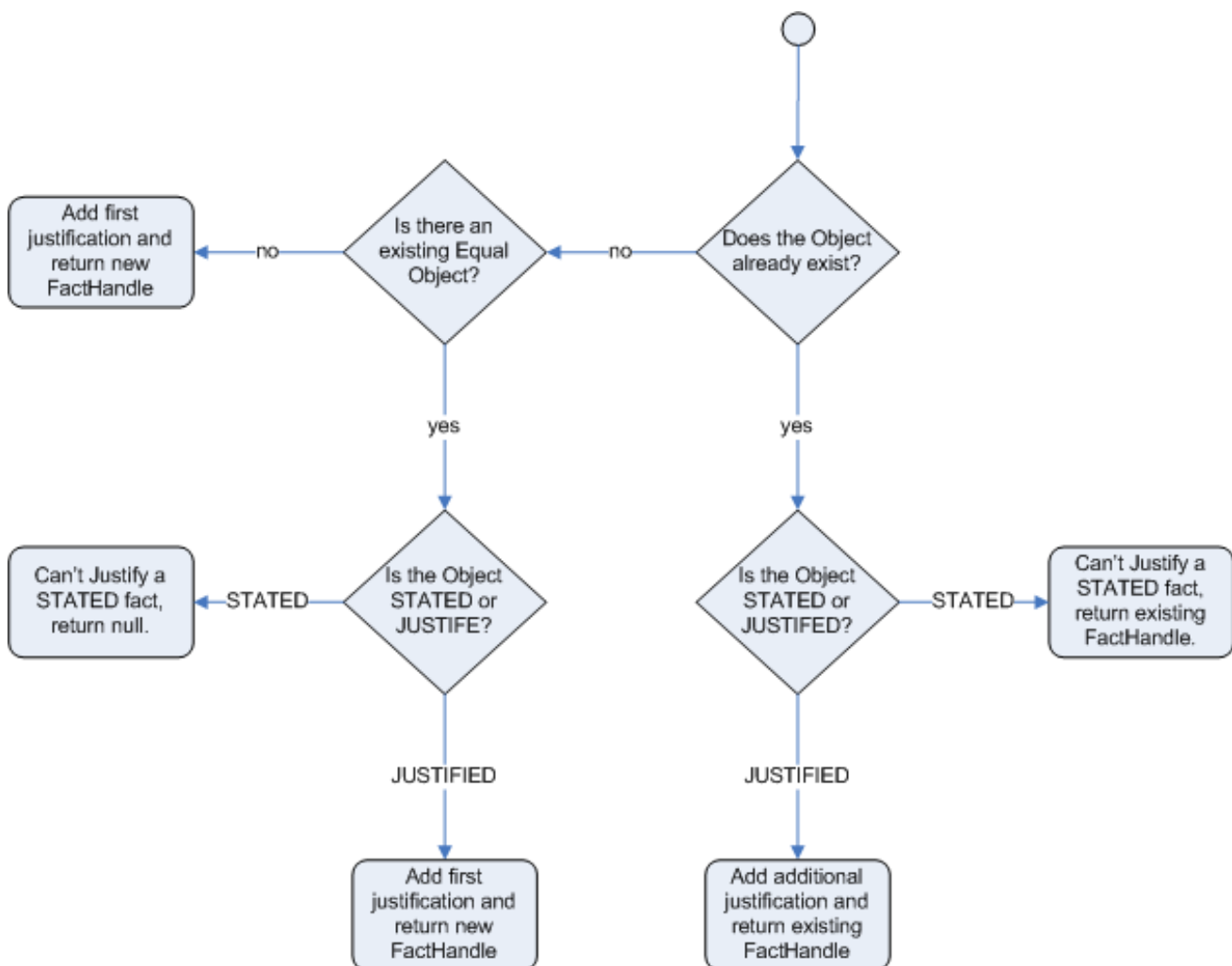
Figure 6.2. Logical Assertion
