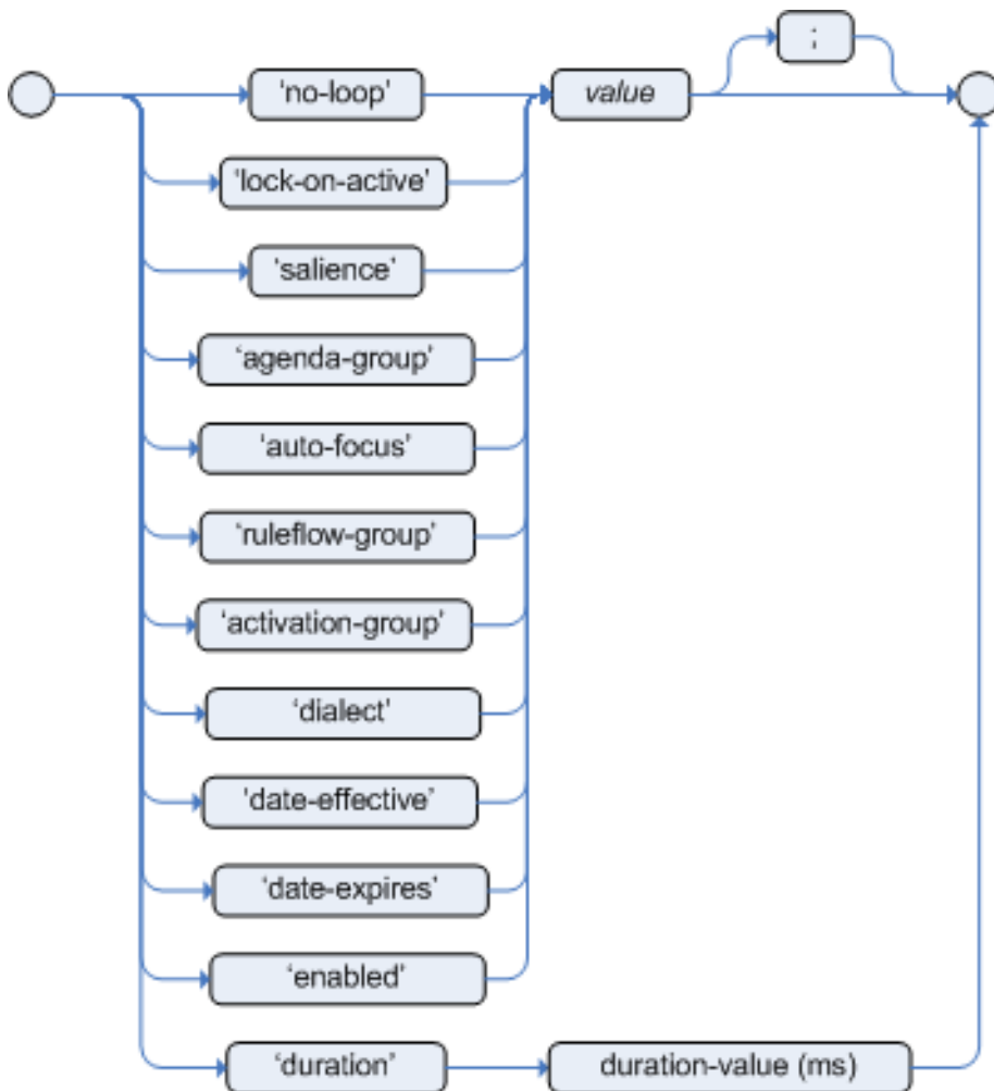
Figure 8.1. Rule Attributes
