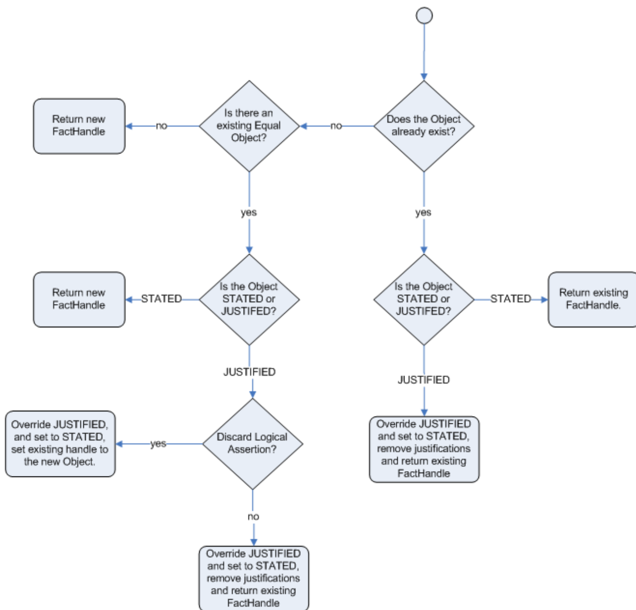
Figure 6.1. Stated Assertion
