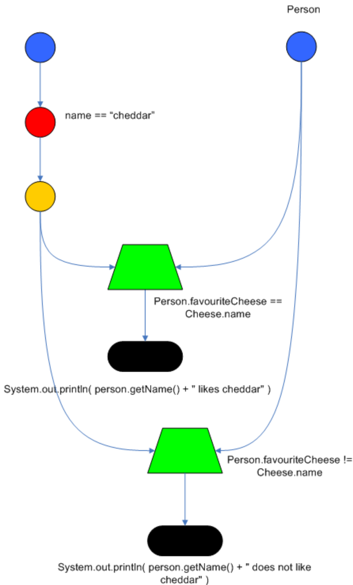
Figure 5.2. Node Sharing
