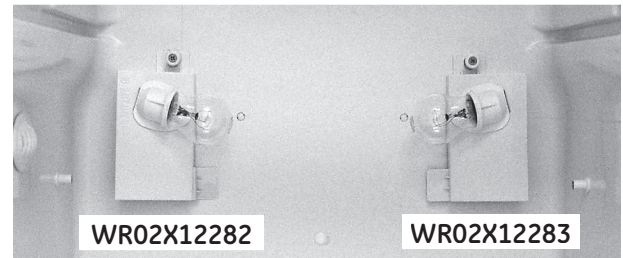
Models 2 plastic reflector facing inward with double sided tape attached to the bottom tab.
