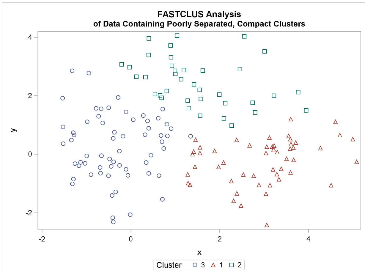
Figure 11.3 Data Containing Poorly Separated, Compact Clusters: PROC FASTCLUS
