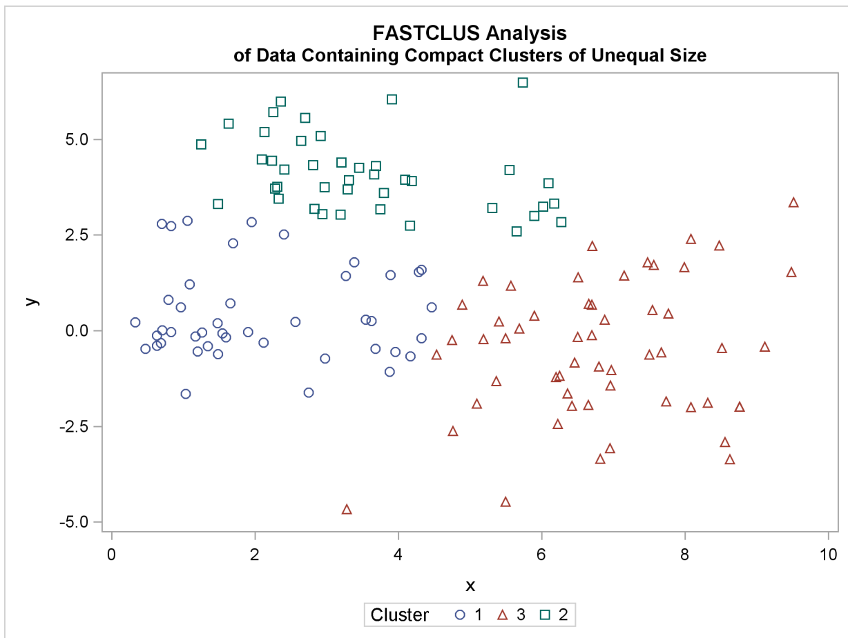
Figure 11.11 Data Containing Compact Clusters of Unequal Size: PROC FASTCLUS
