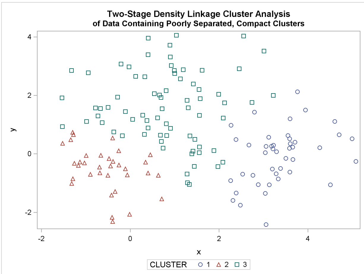
Figure 11.7 Data Containing Poorly Separated, Compact Clusters: PROC CLUSTER with METHOD=TWOSTAGE
