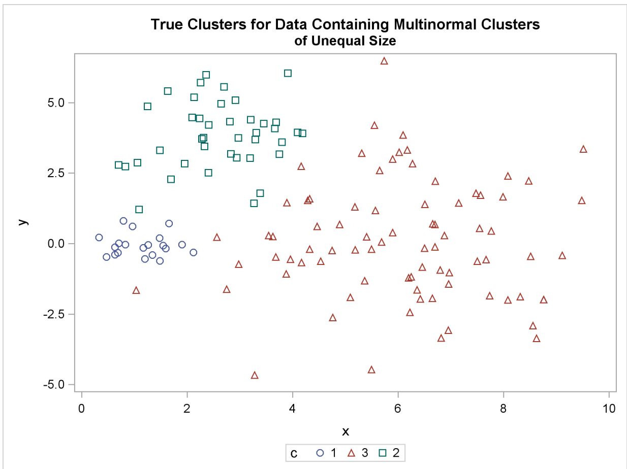
Figure 11.10 Data Containing Generated Clusters of Unequal Size
