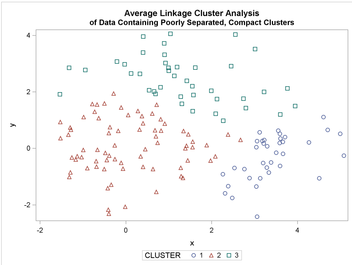
Figure 11.5 Data Containing Poorly Separated, Compact Clusters: PROC CLUSTER with METHOD=AVERAGE
