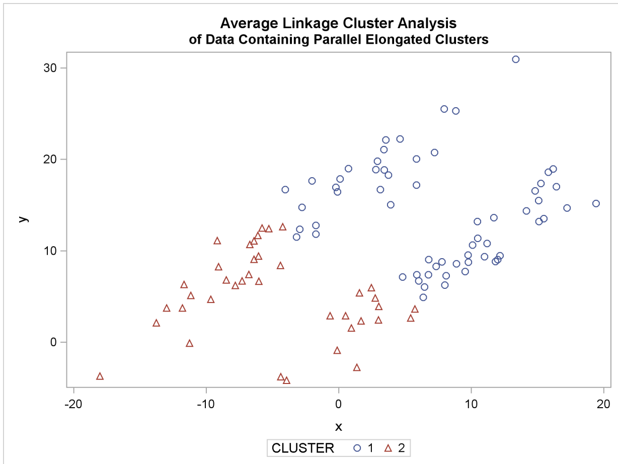
Figure 11.19 Data Containing Parallel Elongated Clusters: PROC CLUSTER with METHOD=AVERAGE
