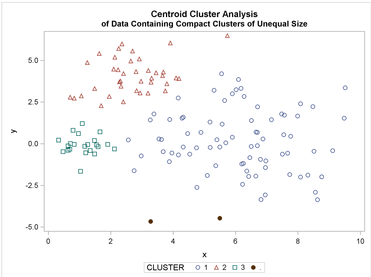
Figure 11.14 Data Containing Compact Clusters of Unequal Size: PROC CLUSTER with METHOD=CENTROID
