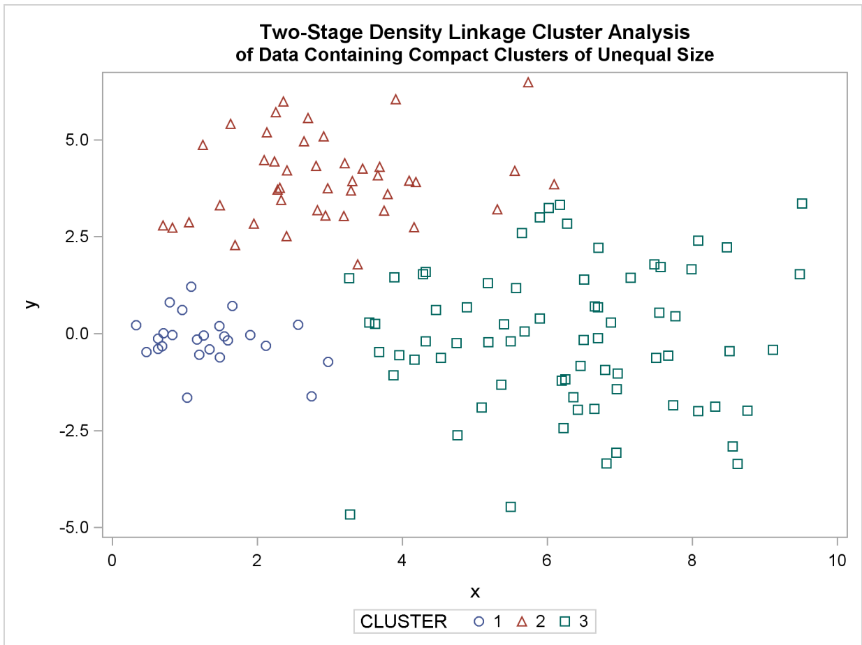
Figure 11.15 Data Containing Compact Clusters of Unequal Size: PROC CLUSTER with METHOD=TWOSTAGE
