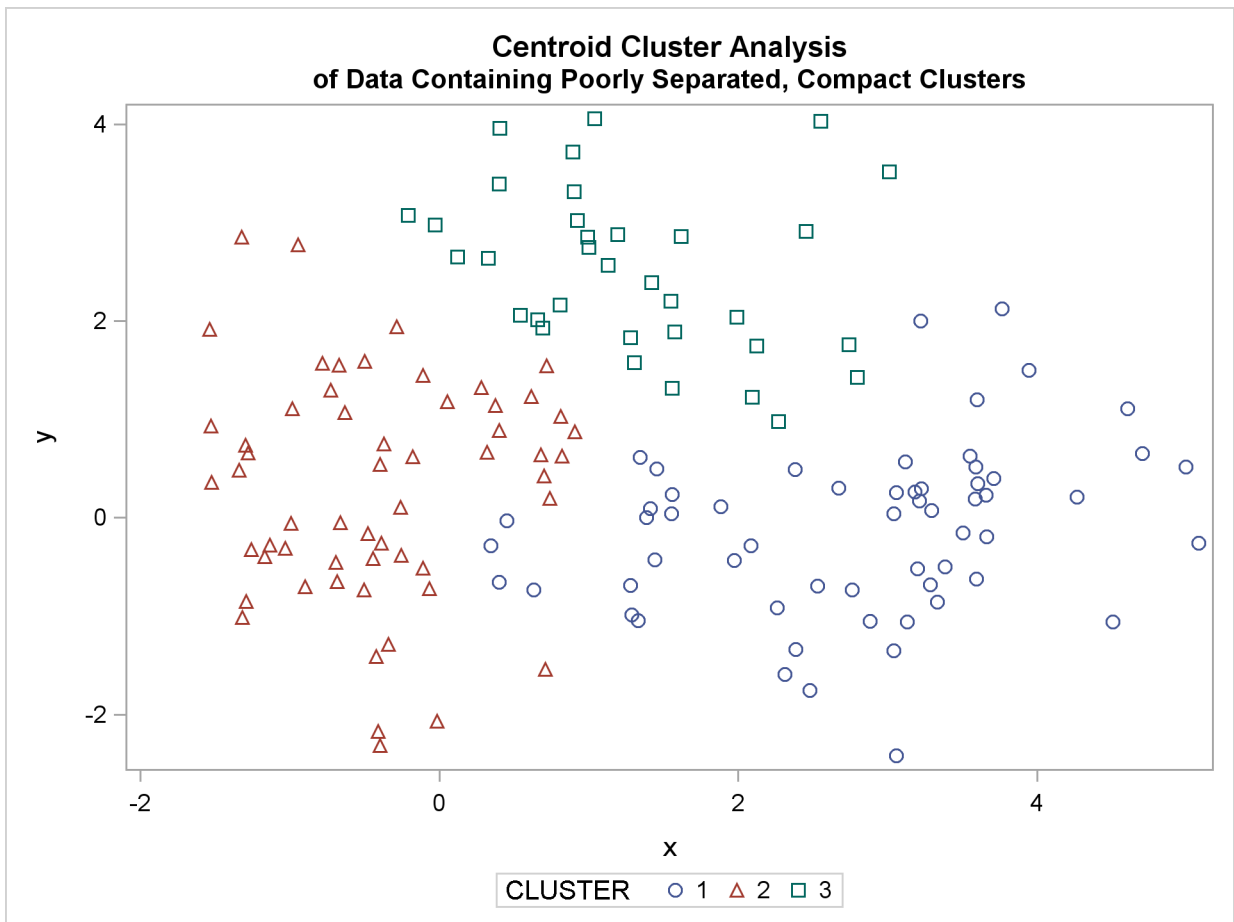
Figure 11.6 Data Containing Poorly Separated, Compact Clusters: PROC CLUSTER with METHOD=CENTROID
