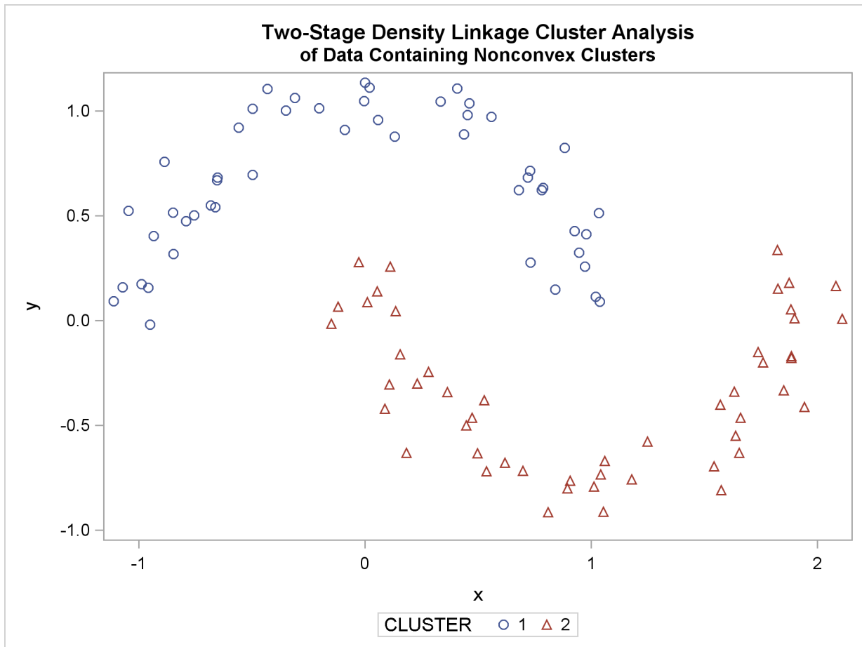
Figure 11.26 Data Containing Nonconvex Clusters: PROC CLUSTER with METHOD=TWOSTAGE
