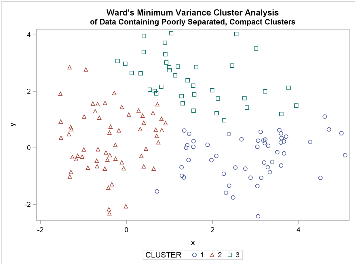
Figure 11.4 Data Containing Poorly Separated, Compact Clusters: PROC CLUSTER with METHOD=WARD
