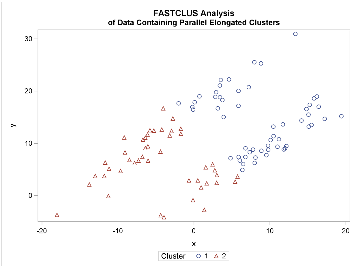
Figure 11.18 Data Containing Parallel Elongated Clusters: PROC FASTCLUS
