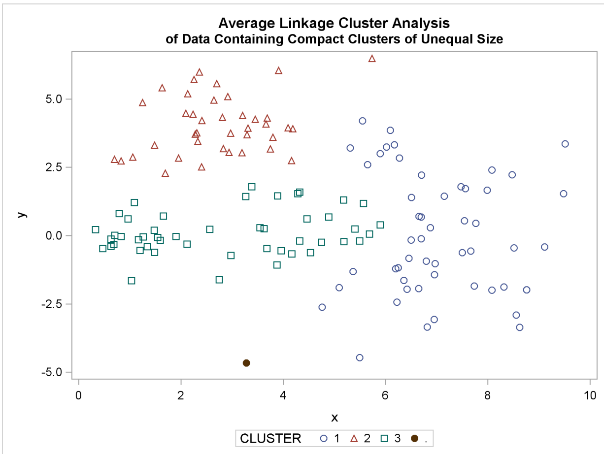
Figure 11.13 Data Containing Compact Clusters of Unequal Size: PROC CLUSTER with METHOD=AVERAGE
