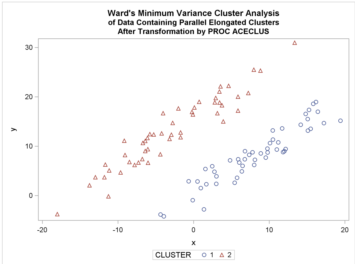
Figure 11.23 Transformed Data Containing Parallel Elongated Clusters: PROC CLUSTER with METHOD=WARD
