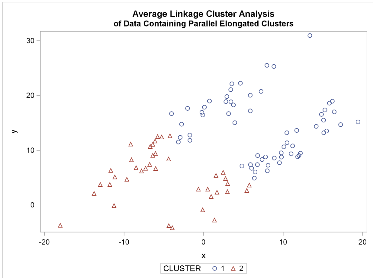
Figure 11.20 Data Containing Parallel Elongated Clusters: PROC CLUSTER with METHOD=TWOSTAGE
