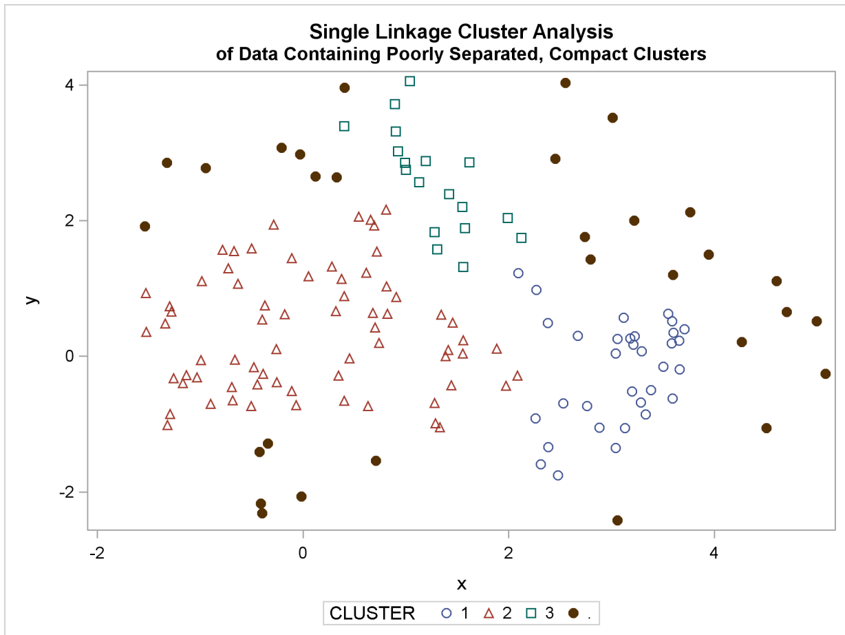
Figure 11.9 Data Containing Poorly Separated, Compact Clusters: PROC CLUSTER with METHOD=SINGLE
