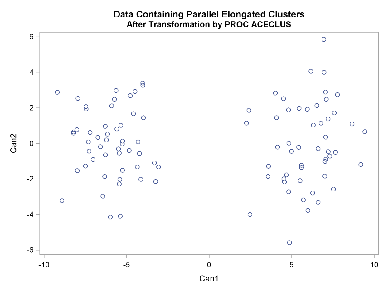
Figure 11.22 Data Containing Parallel Elongated Clusters after Transformation by PROC ACECLUS
