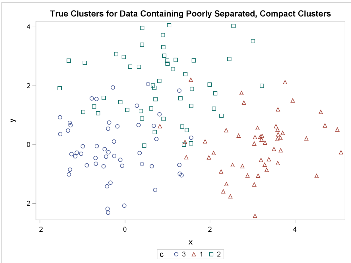
Figure 11.2 Data Containing Poorly Separated, Compact Clusters: Plot of True Clusters
