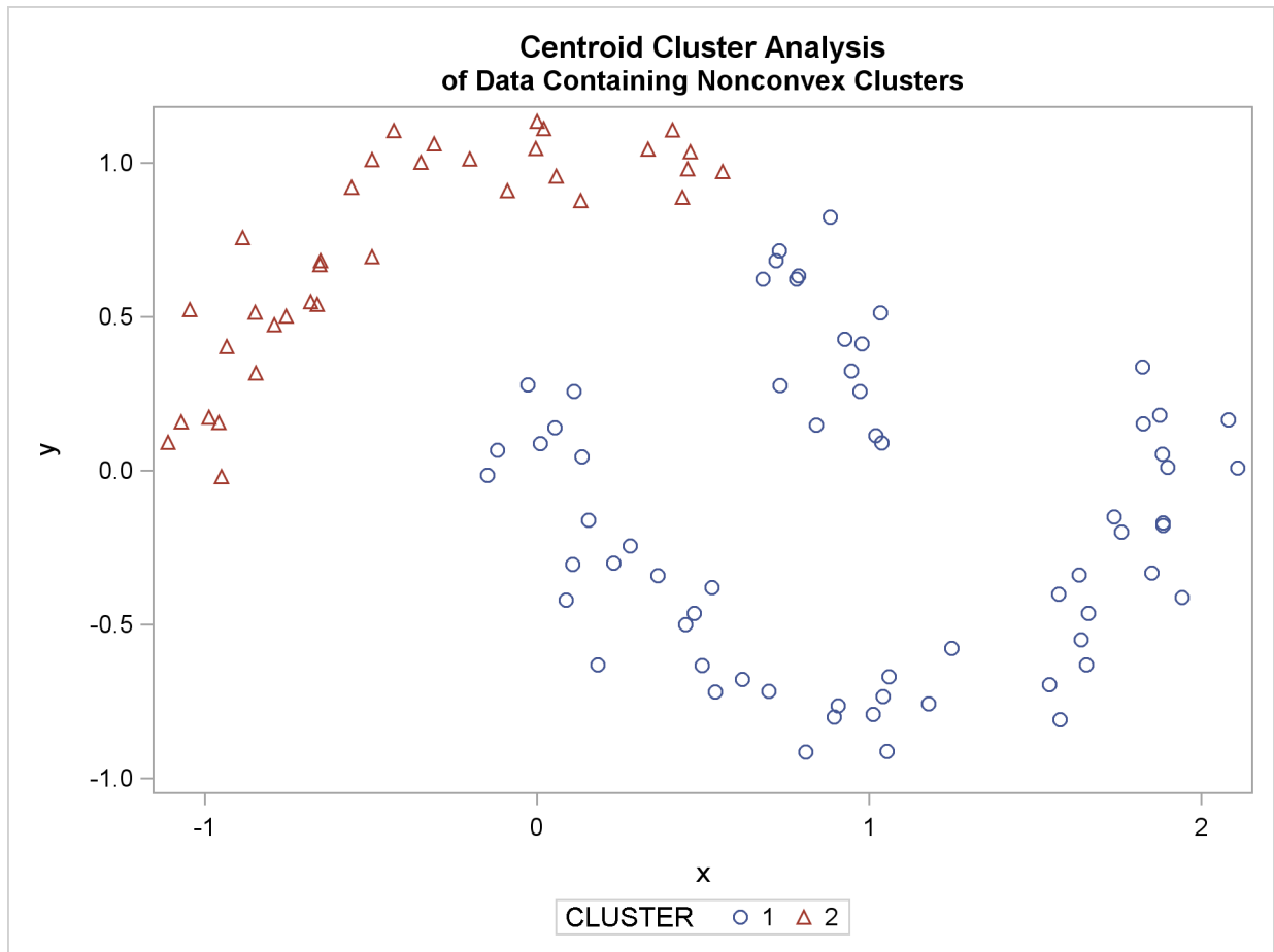
Figure 11.25 Data Containing Nonconvex Clusters: PROC CLUSTER with METHOD=CENTROID
