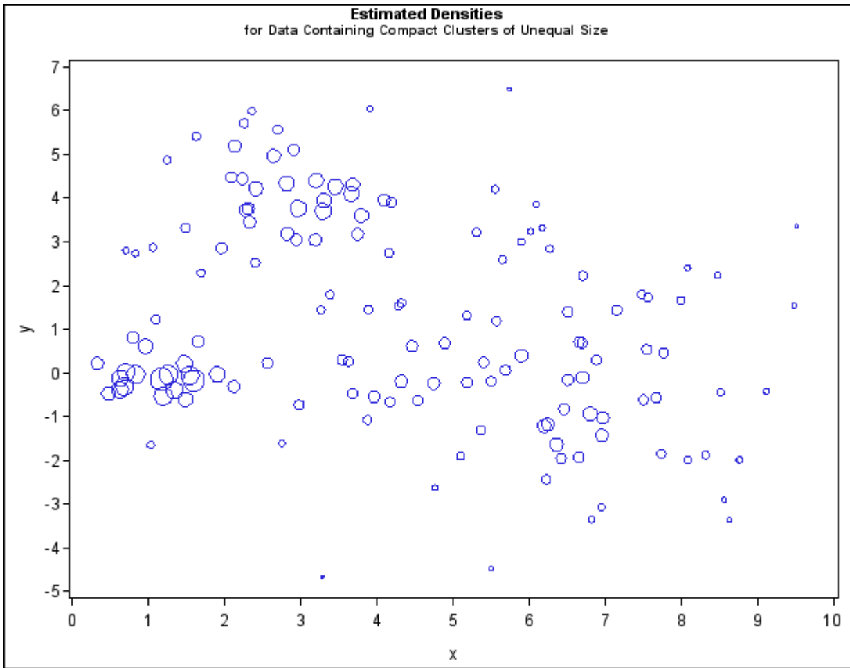
Figure 11.16 Data Containing Compact Clusters of Unequal Size: PROC CLUSTER with METHOD=TWOSTAGE
