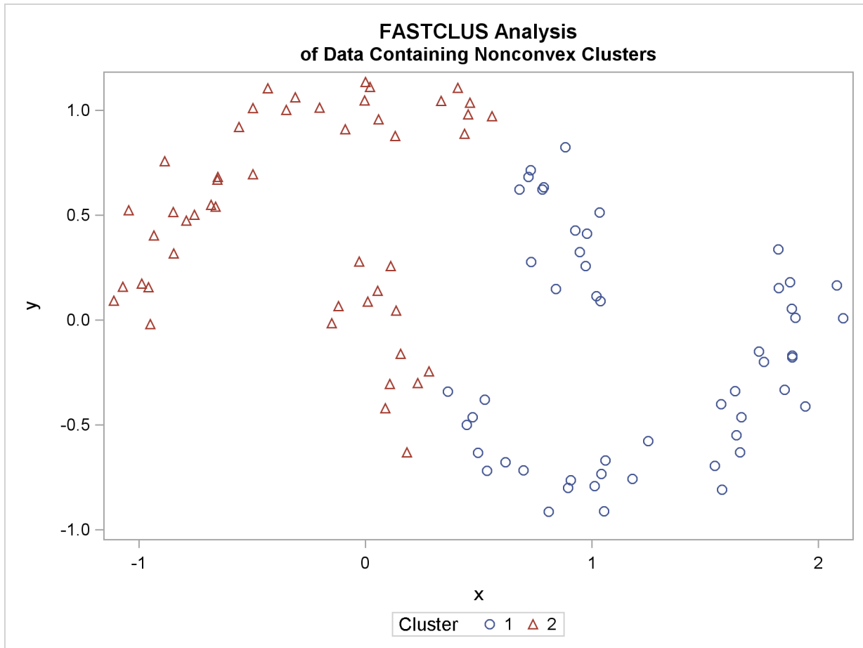
Figure 11.24 Data Containing Nonconvex Clusters: PROC FASTCLUS
