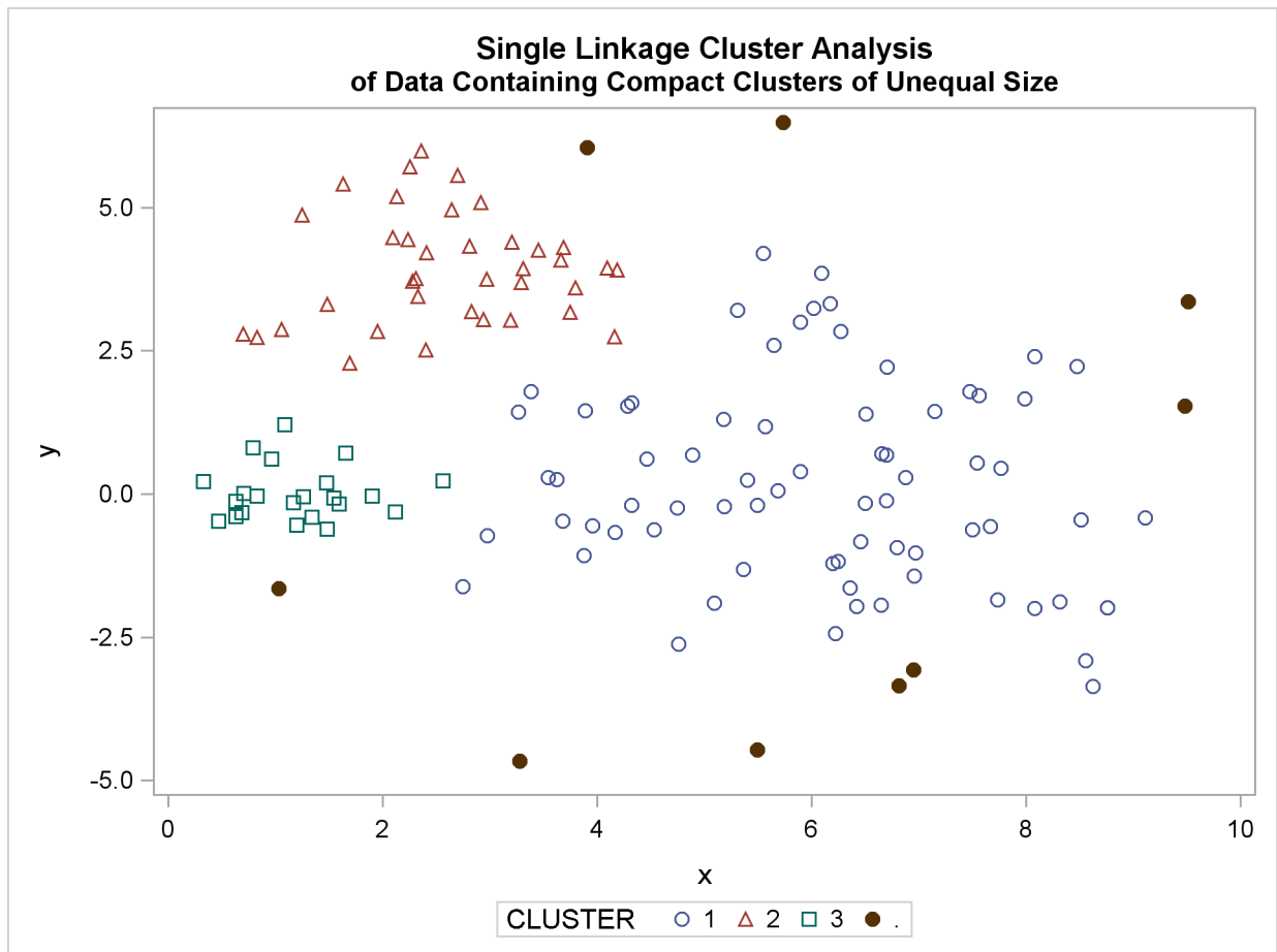
Figure 11.17 Data Containing Compact Clusters of Unequal Size: PROC CLUSTER with METHOD=SINGLE
