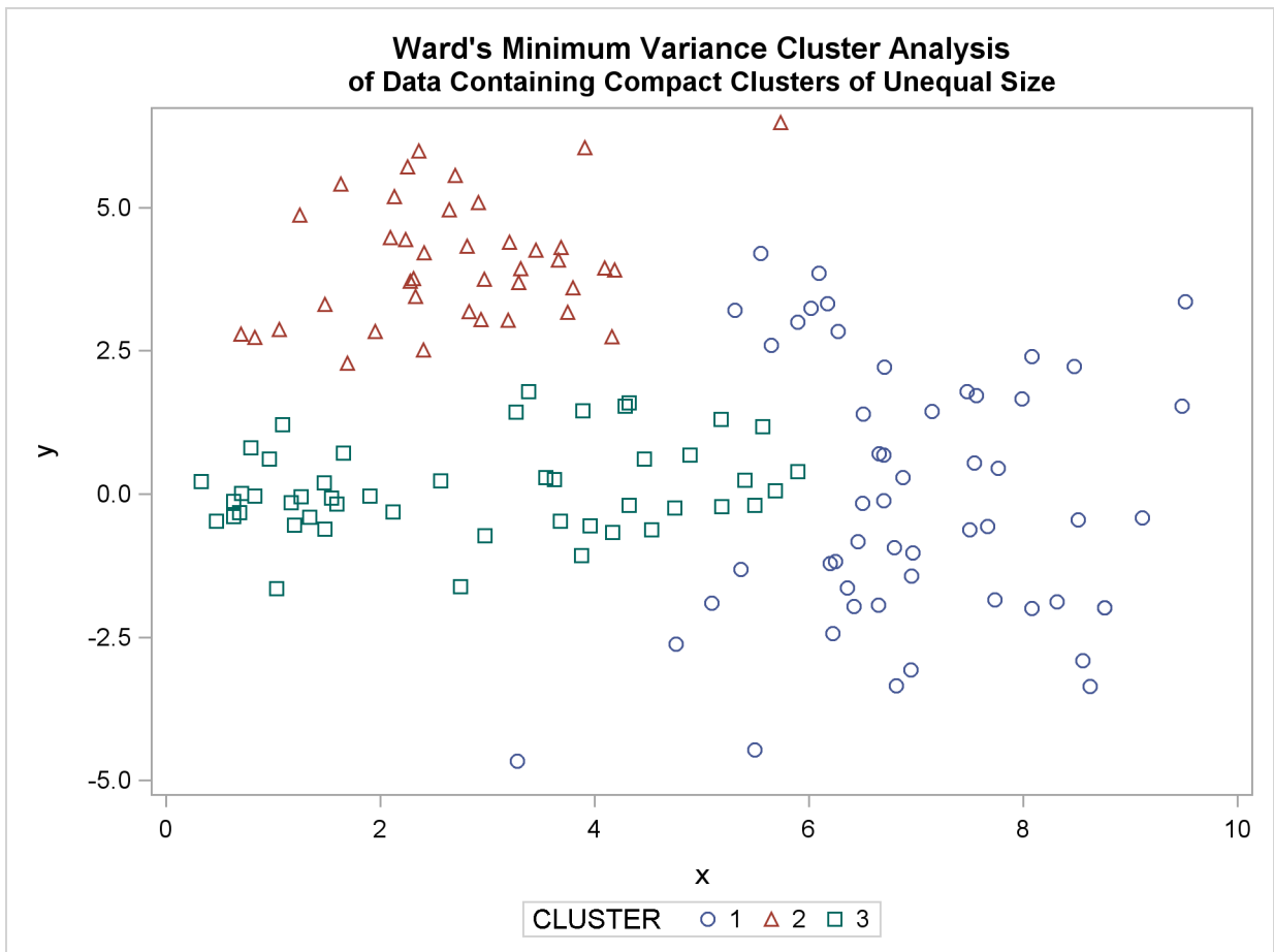
Figure 11.12 Data Containing Compact Clusters of Unequal Size: PROC CLUSTER with METHOD=WARD
