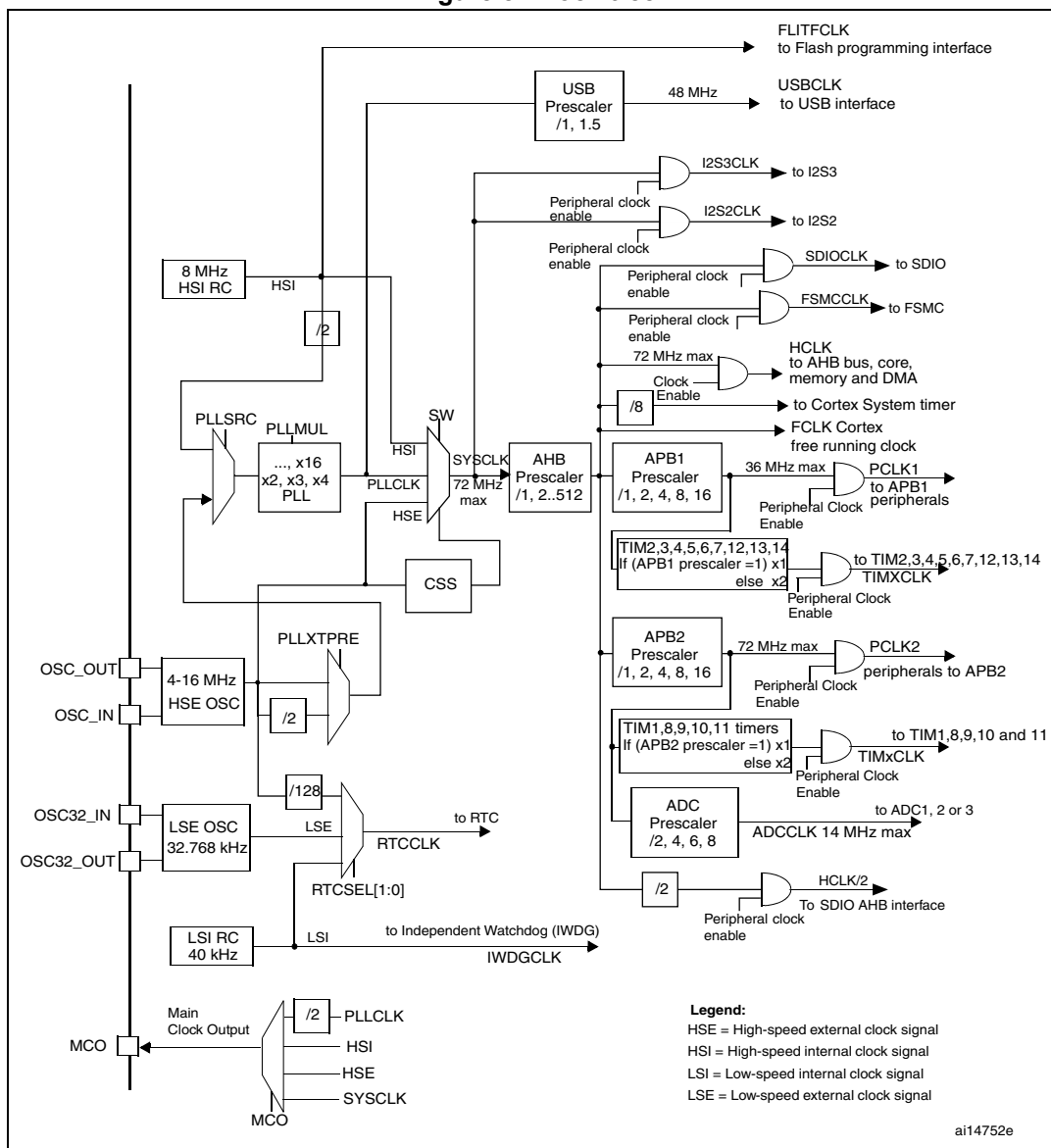
Figure 8. Clock tree
