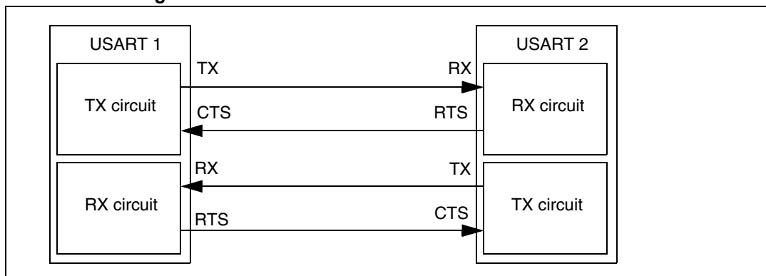
Figure 298. Hardware flow control between two USARTs
