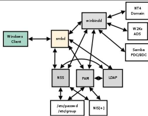
Figure 7.3. Samba and Authentication Backend Search Pathways
