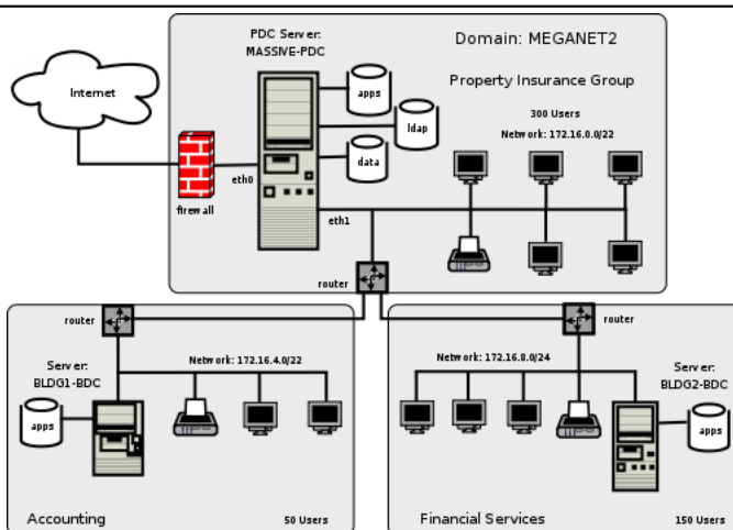
Figure 6.2. Network Topology 500 User Network Using ldapsam passdb backend.
