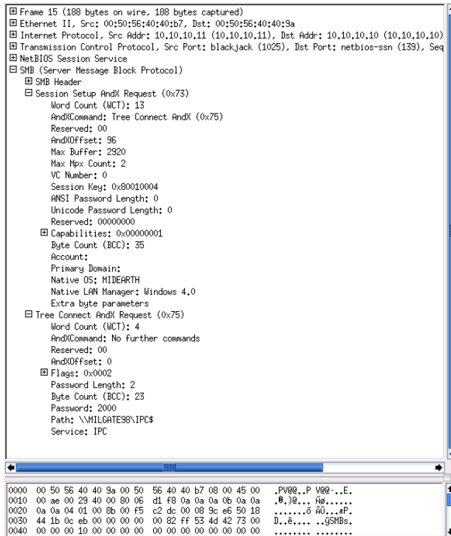
Figure 1.4. Typical Windows 9x/Me NULL SessionSetup AndX Request
