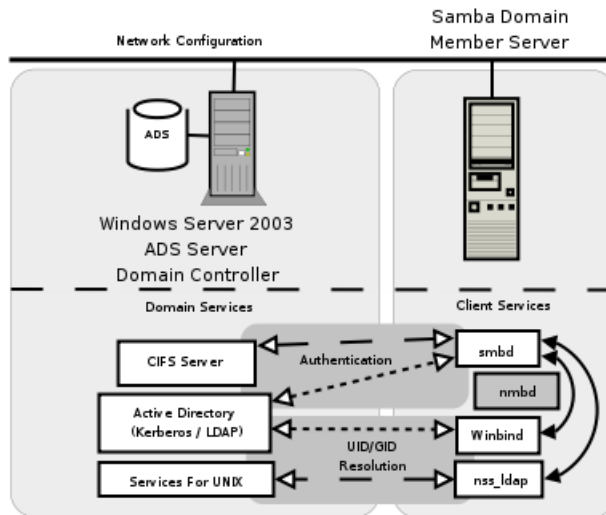
Figure 10.3. Active Directory Domain: Samba Member Server
