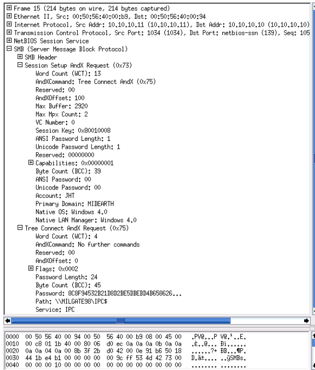
Figure 1.5. Typical Windows 9x/Me User SessionSetup AndX Request
