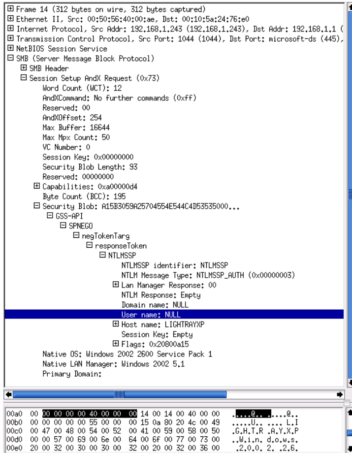
Figure 1.6. Typical Windows XP NULL Session Setup AndX Request
