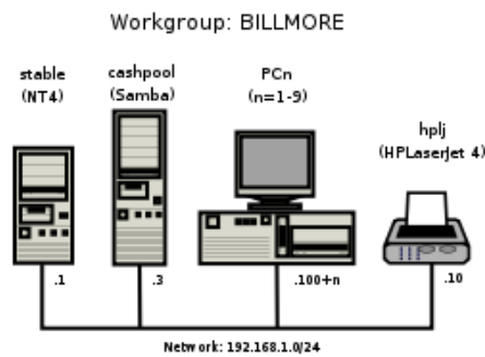
Figure 2.2. Accounting Office Network Topology
