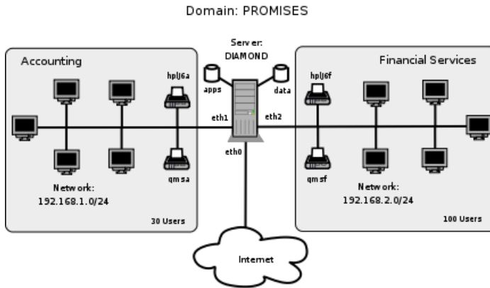
Figure 4.1. Abmas Network Topology 130 Users
