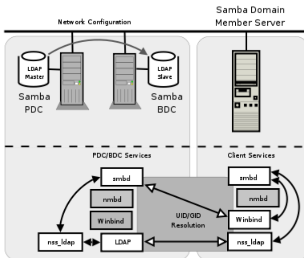
Figure 10.2. Samba Domain: Samba Member Server
