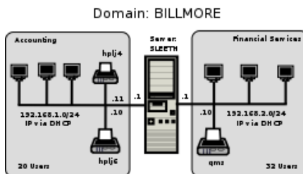
Figure 3.1. Abmas Accounting 52 User Network Topology
