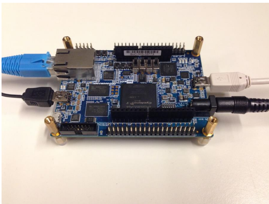
Figure 9-18. DE0-Nano-SoC Wiring
