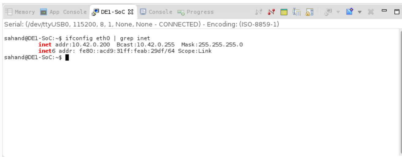
Figure 13-16. Obtaining the DE0-Nano-SoC's IP Address through ARM DS-5's Serial Terminal
