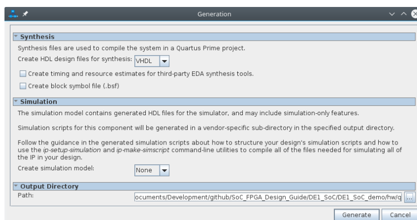
Figure 9-15. Generate Qsys System
