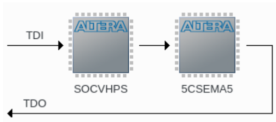
Figure 9-22. JTAG Scan Chain
