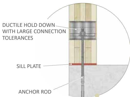
CLT Hold Down Connection
