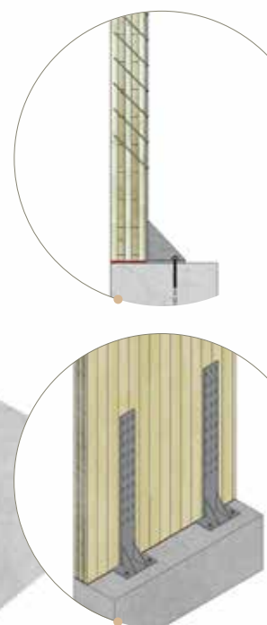
High Force Hold Down Connection
