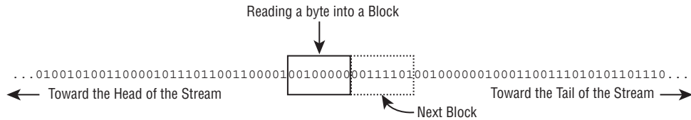
FIGURE 8.2 Visual representation of a stream
