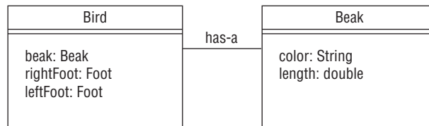
FIGURE 2.8 Bird has-a Beak.
