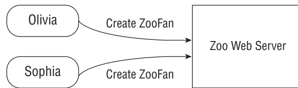
FIGURE 7.5 Race condition on user creation
