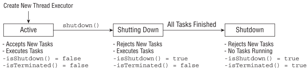
FIGURE 7.2 ExecutorService life cycle
