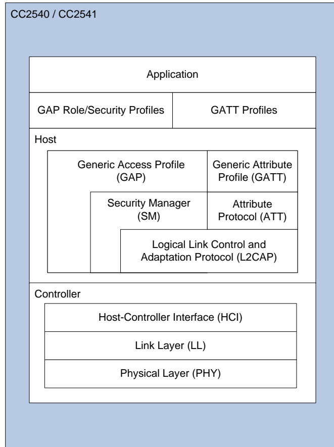
Figure 3: Single-Device Configuration
