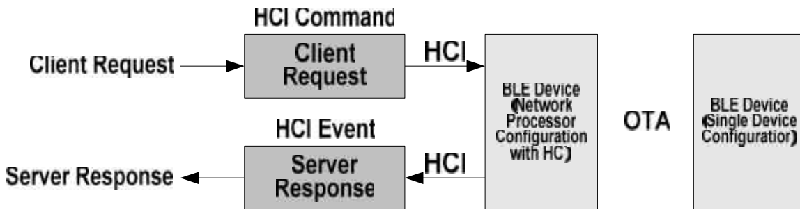
Figure 8: Request/Response with Server Database in BLE Stack
