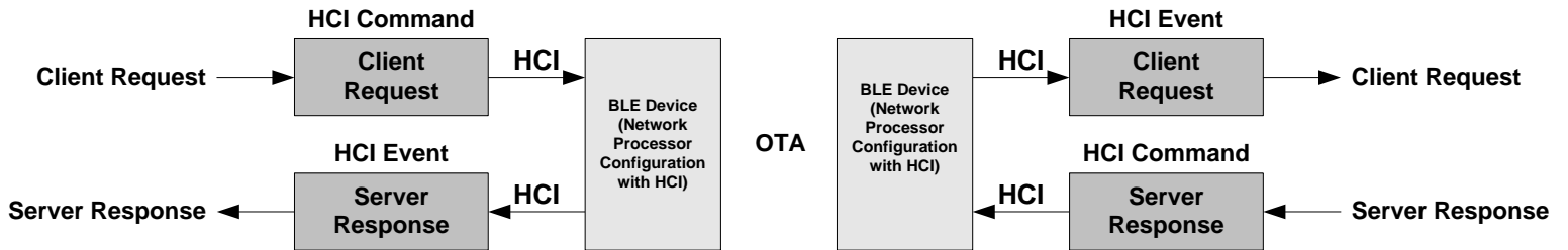
Figure 9: Request/Response with Server Database not in BLE Stack
