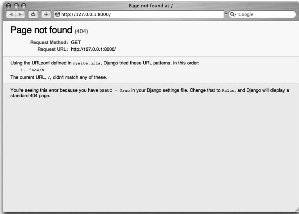
Figure 3-1. Django's 404 page
