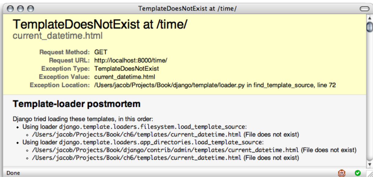
Figure 6.1: Figure 4-1: The error page shown when a template cannot be found.
