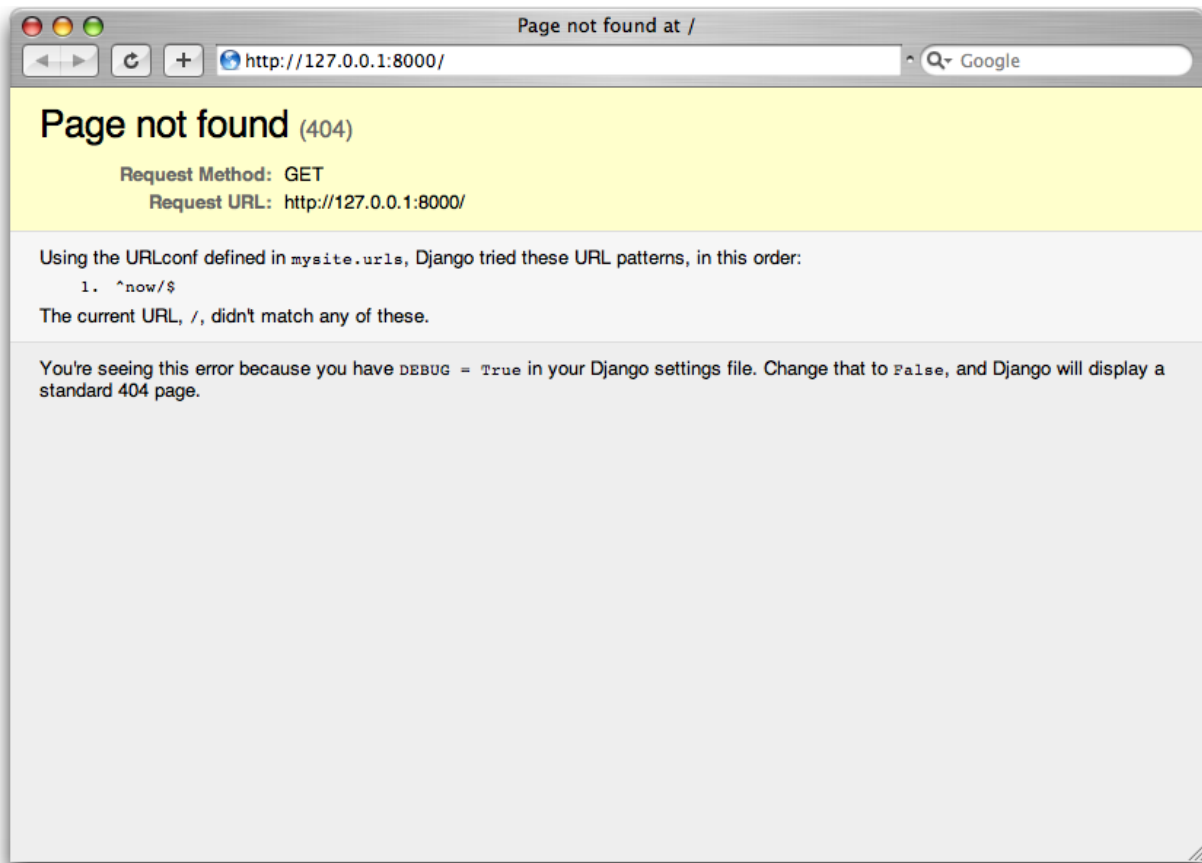
Figure 5.1: Figure 3-1. Django's 404 page
