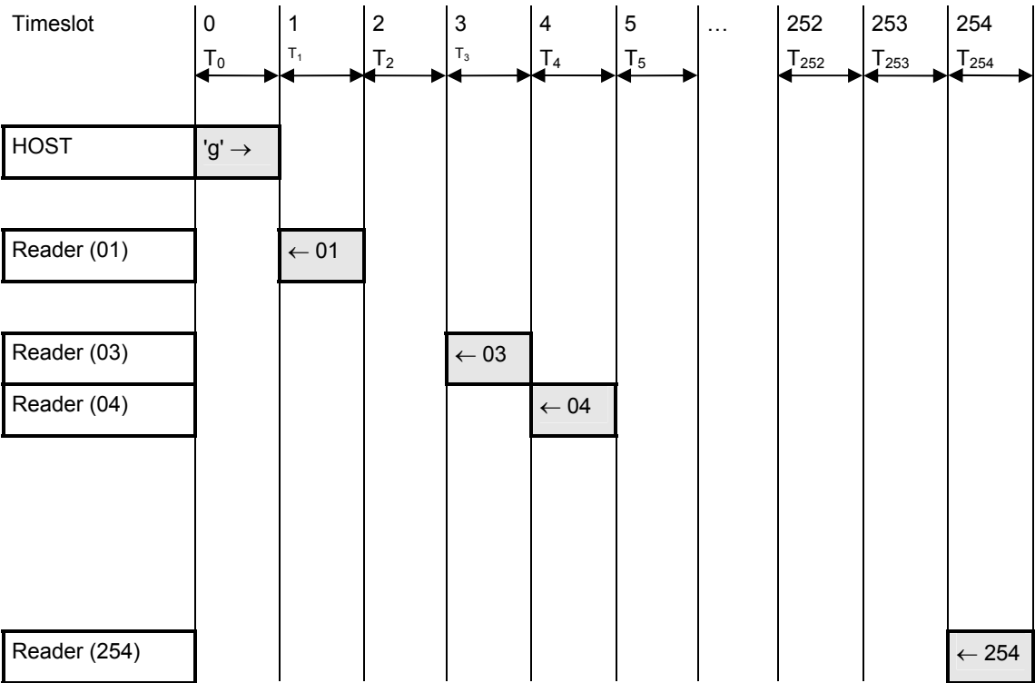
Figure 8 Time slotted answers diagram
