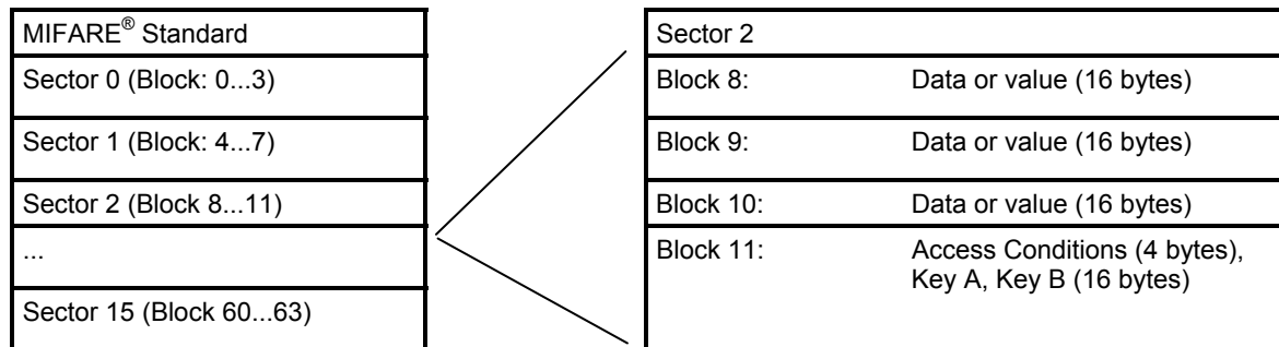
Figure 1 MIFARE® Standard: sector diagram
