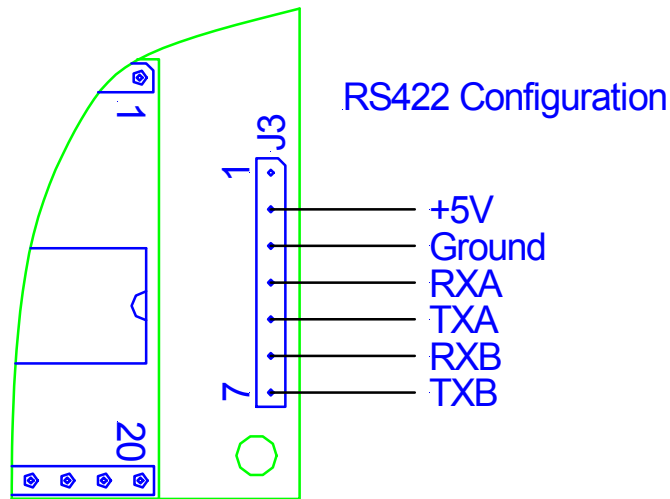
Figure 11 Pin out of jumper 3 in RS422 Configuration
