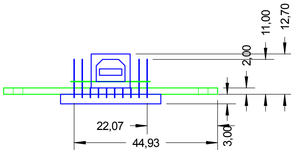
Figure 16 Short Range Plug & Play Module - Front View
