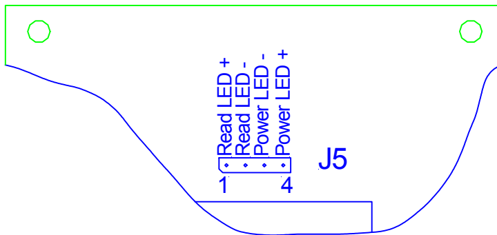
Figure 18 Pin out of Jumper 5 - Top View
