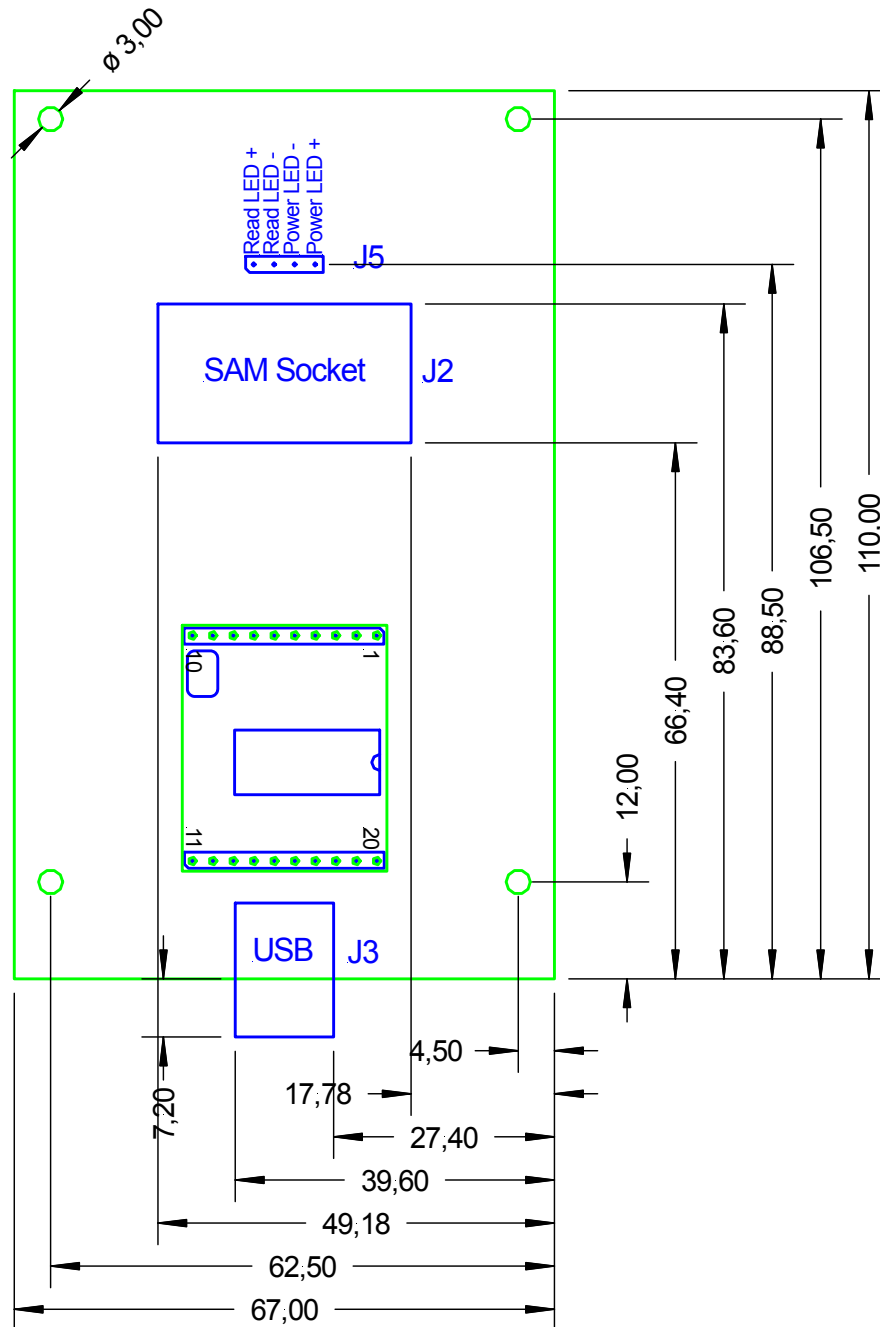
Figure 15 Short Range Plug & Play Module - Top view
