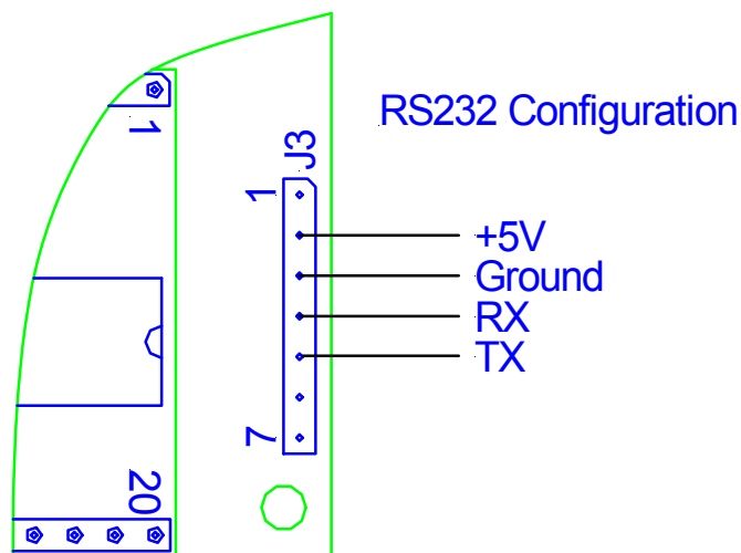
Figure 10 Pin out of jumper 3 in RS232 Configuration
