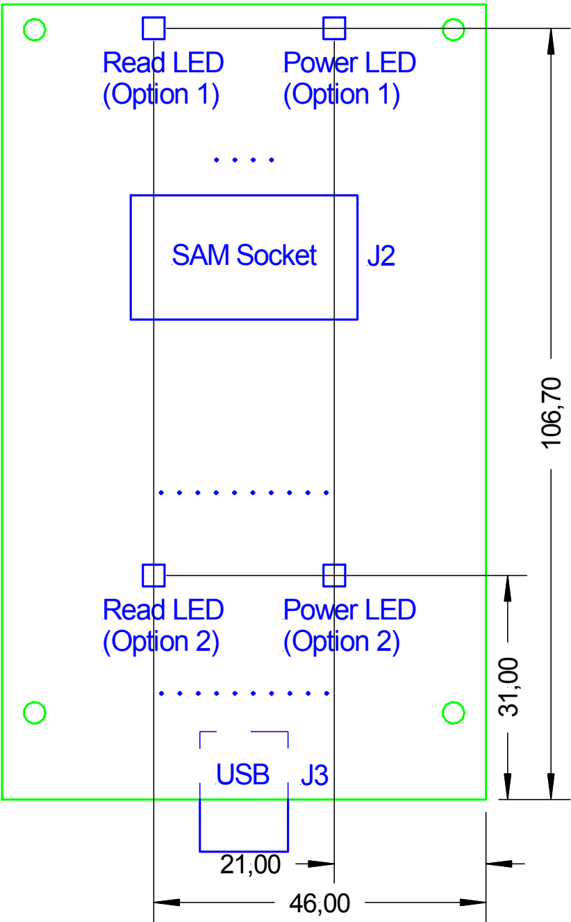
Figure 17 Short Range Plug & Play Module - Bottom View
