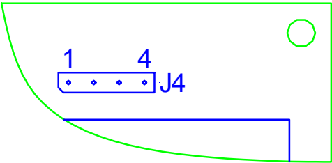
Figure 13 Pin out of Jumper 4 (top view)
