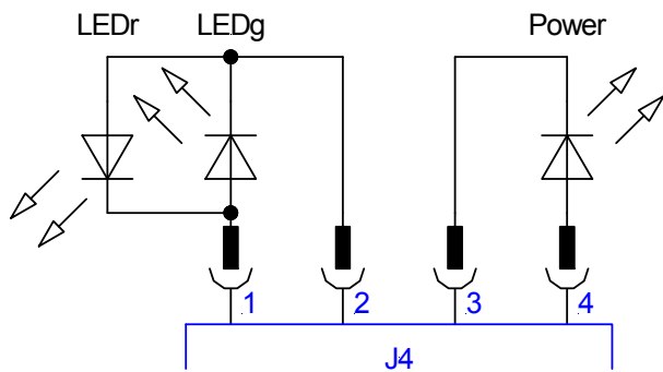
Figure 14 Pin out of jumper 4
