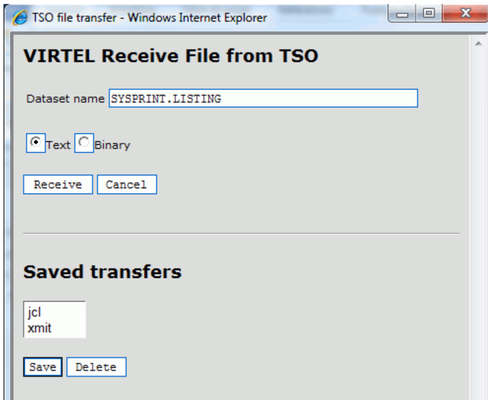
Receive dialog (saved transfers)
