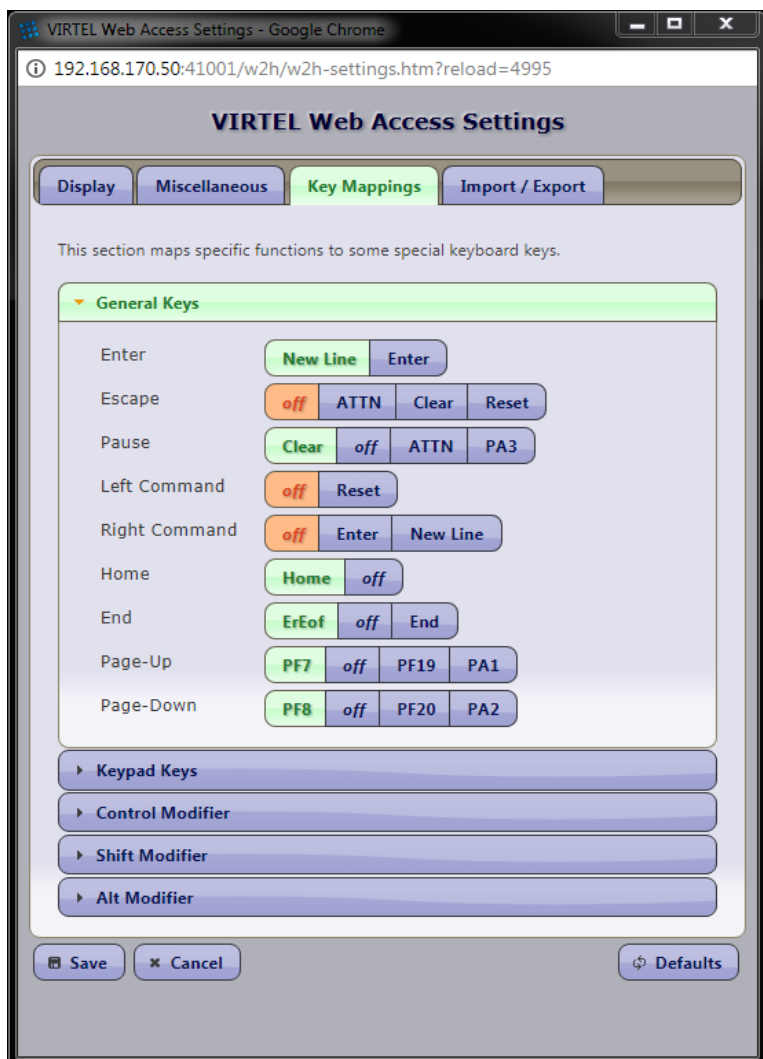
VIRTTEL Web Access Settings Key Mappings Tab (part 3 of 4)
