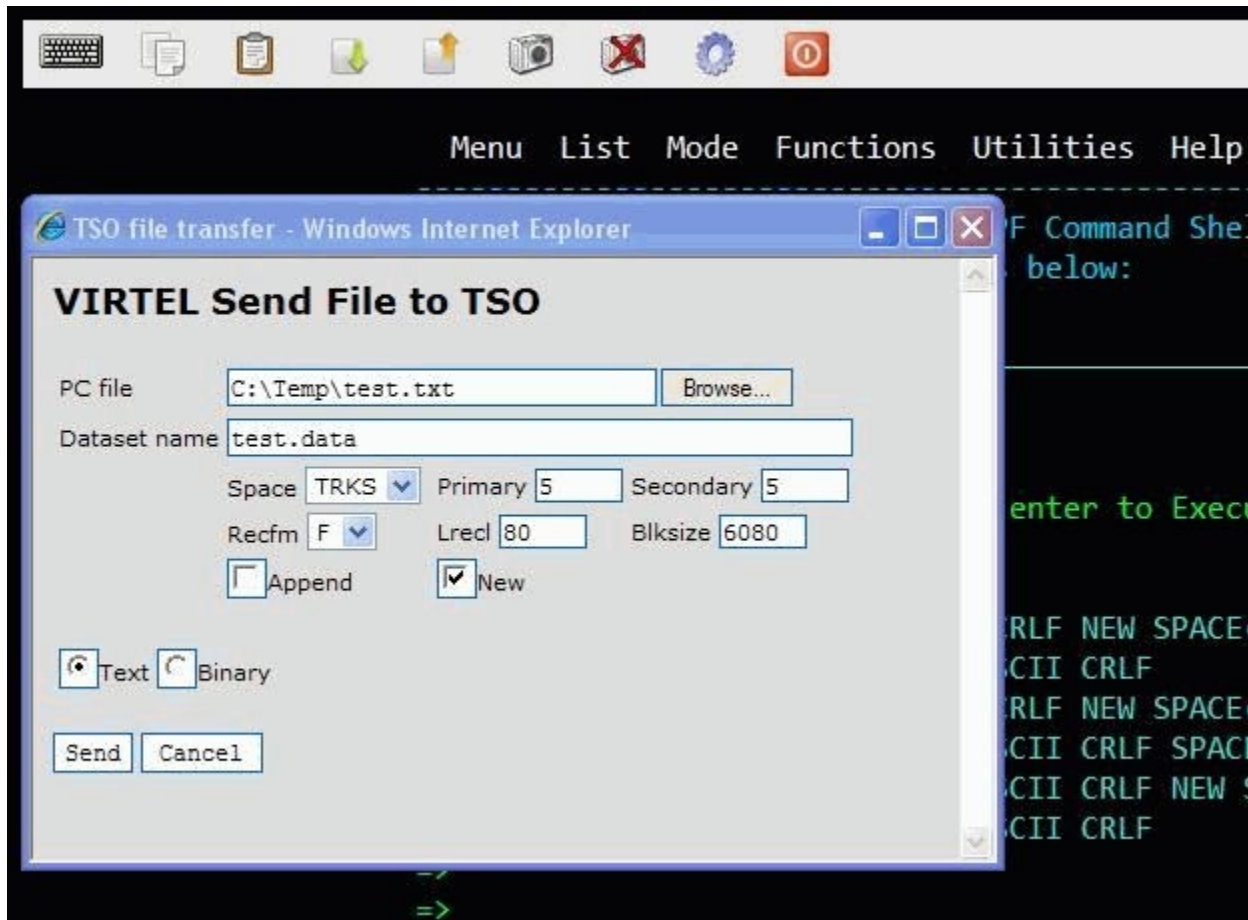
VIRTTEL IND$FILE send dialog (part 3)
