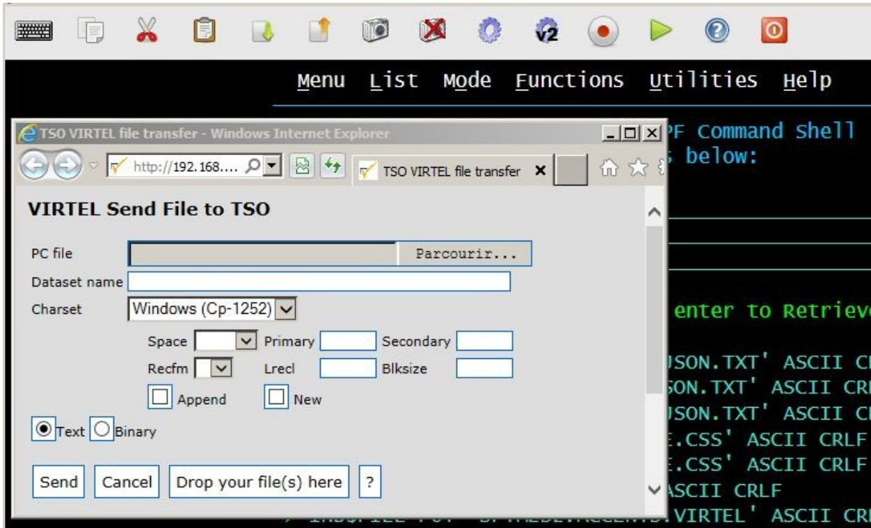
VIRTEL IND$FILE send dialog (part 1)
