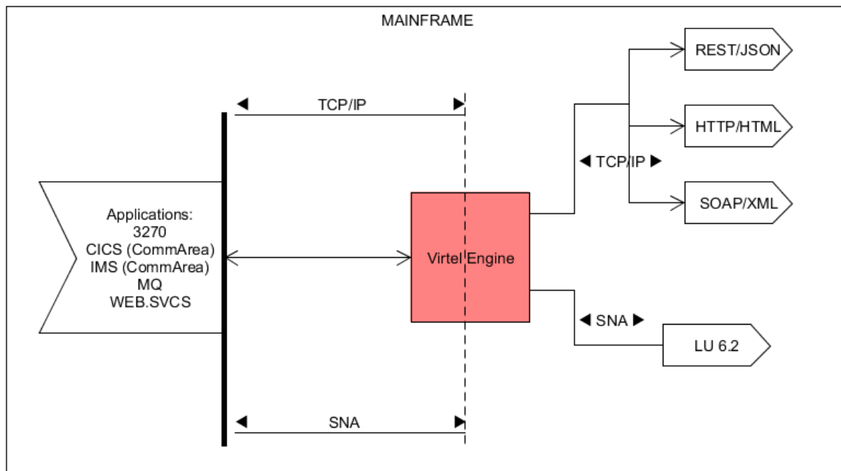
The Virtel Engine
