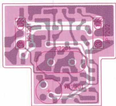
"component" side
