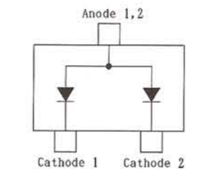
1SS181 (A3) (D3003, 3039, 3053)
