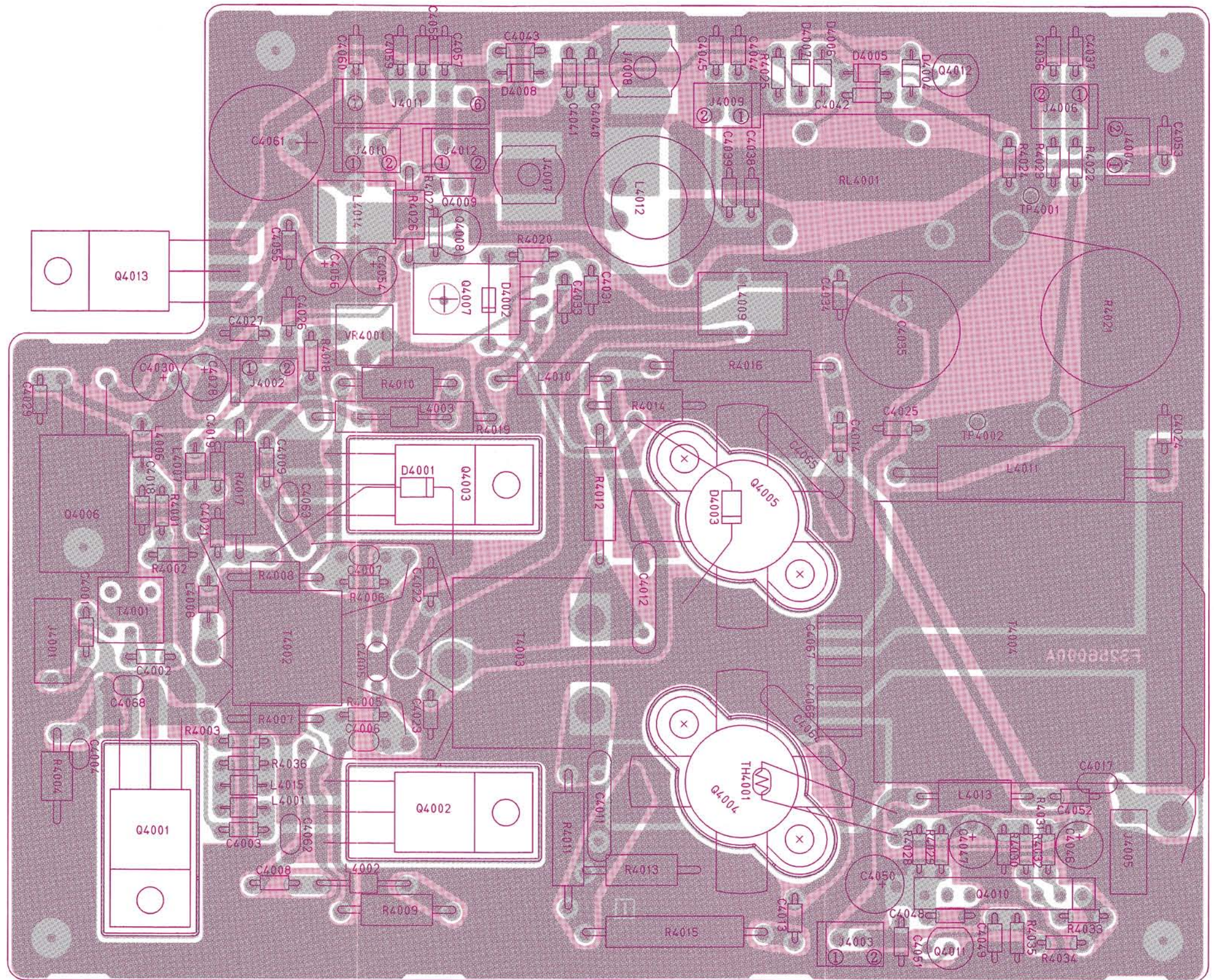
"component" side
