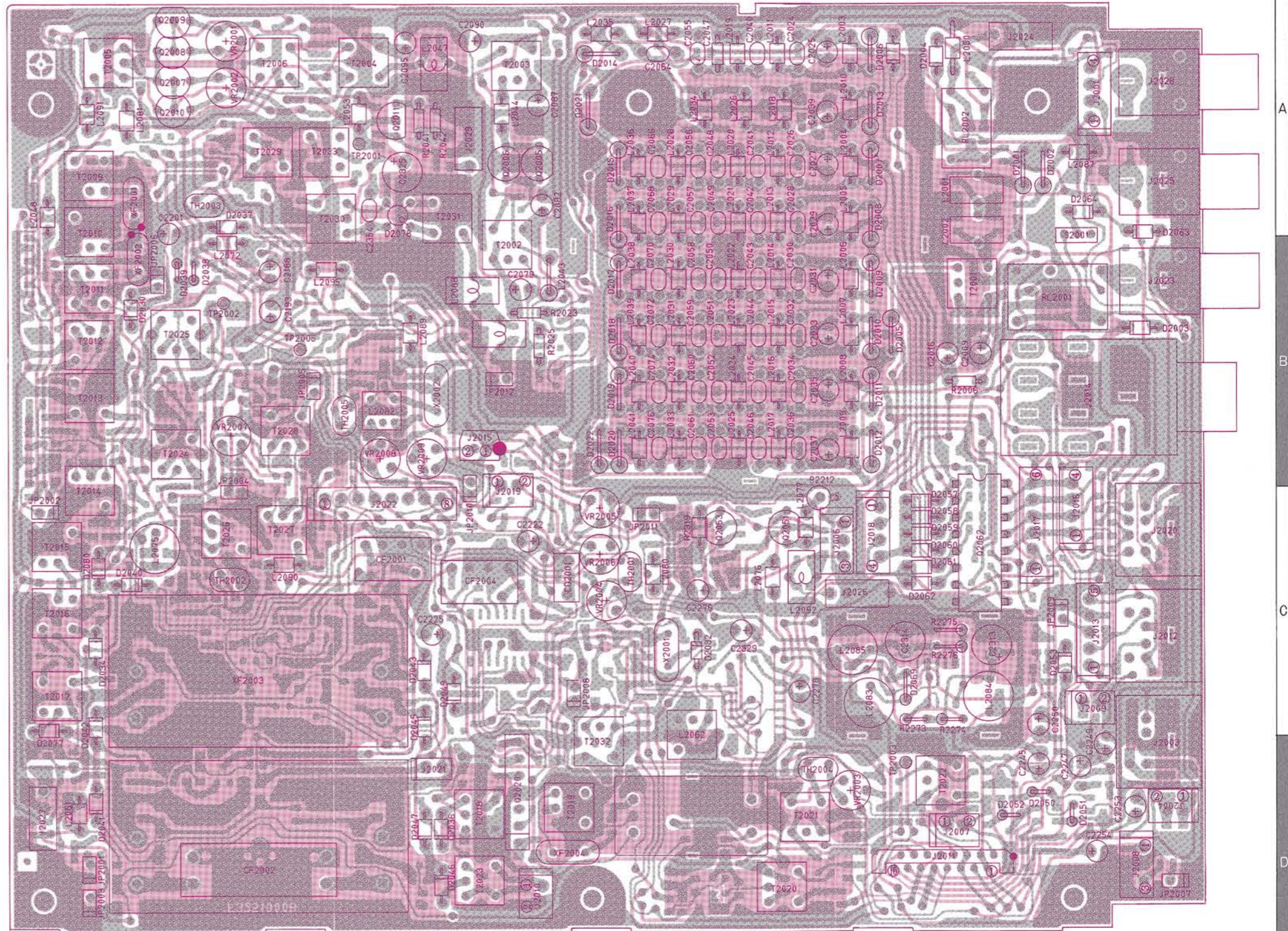
"component" side
