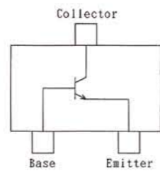
2SC2712GR (LG) (Q7001, 7002)
