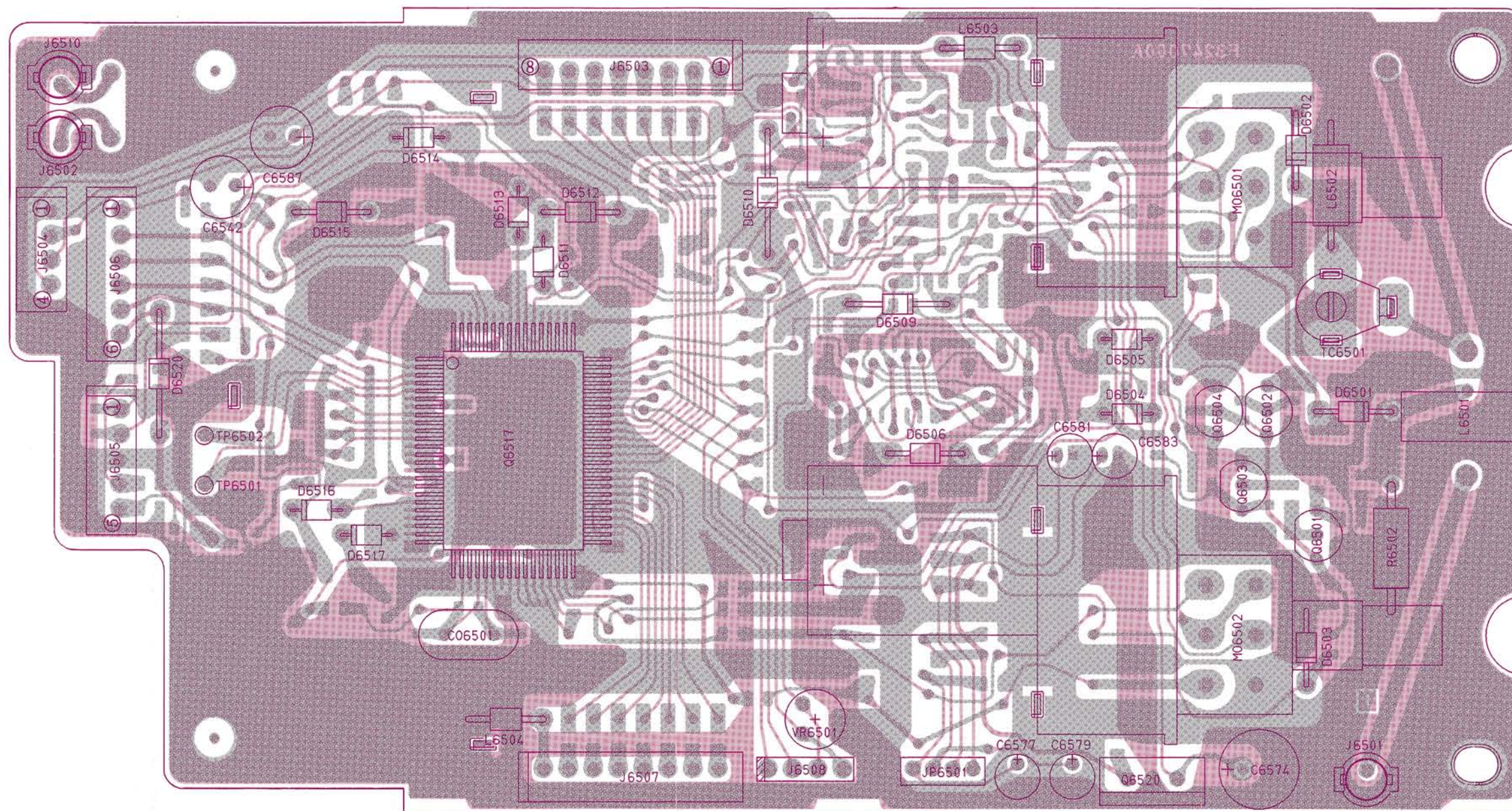
"component" side
