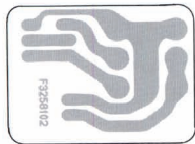
"solder" side
