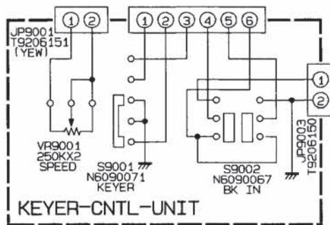
"solder" side
