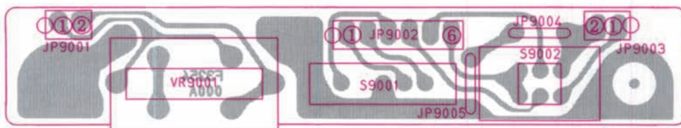
"component" side
