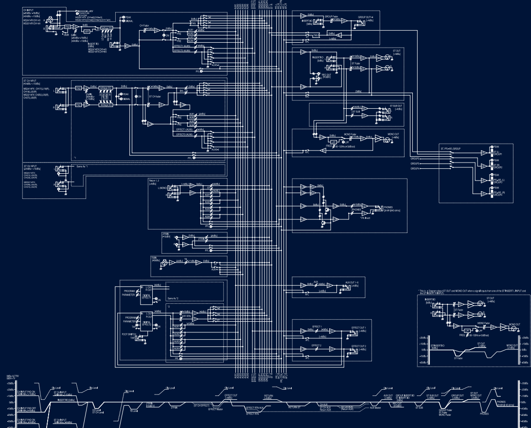
MG24/14FX, MG32/14FX Block and Level Diagram
