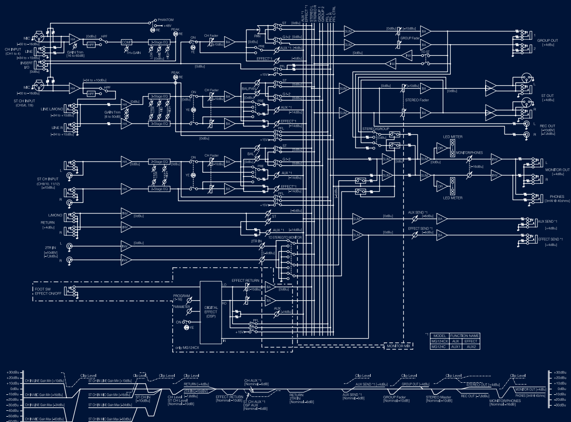
MG124C, MG124CX Block and Level Diagram
