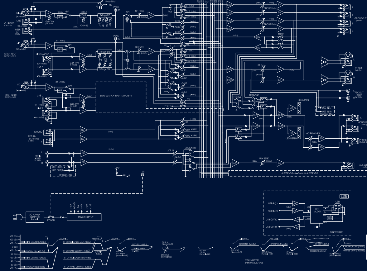
MG206C, MG206C-USB Block and Level Diagram
