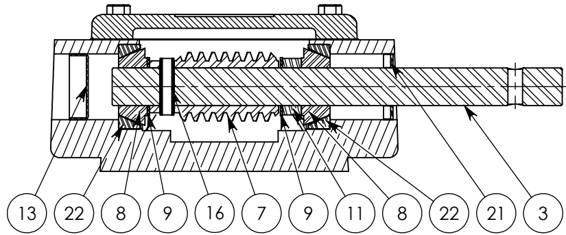
SECTION B-B
