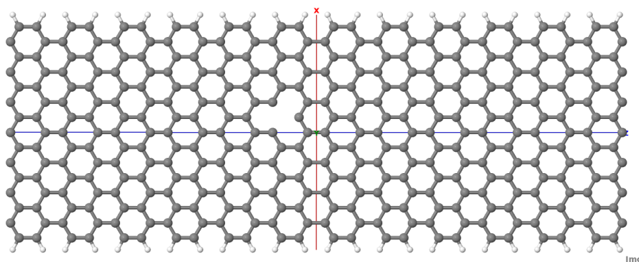
Fig. 4.7: Geometry with vacancy on sublattice A
