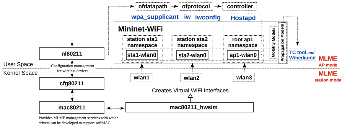
Figure 1.1: Mininet-WiFi Components.
