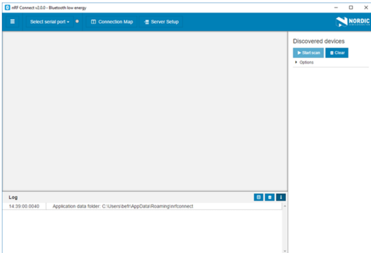
Figure 1: Application window
