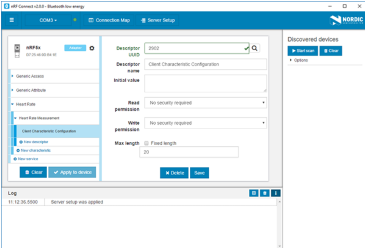
Figure 5: Server setup
