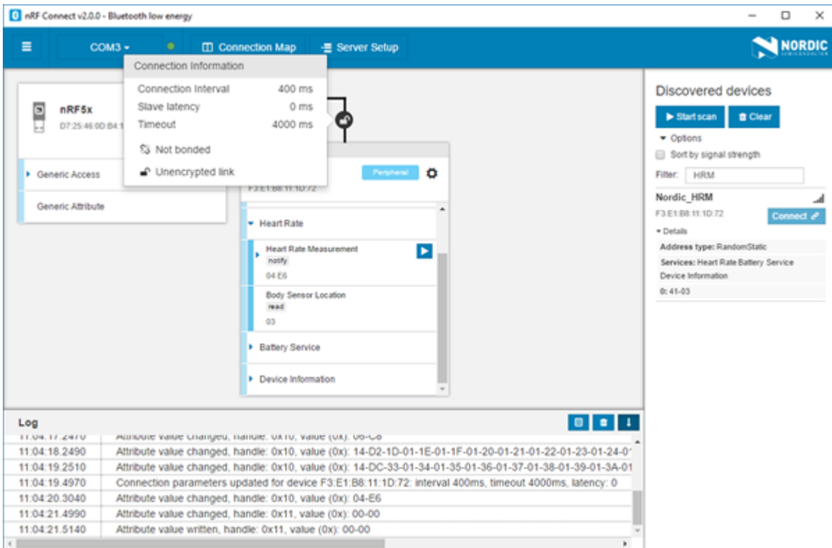
Figure 4: Hovering over the padlock icon
