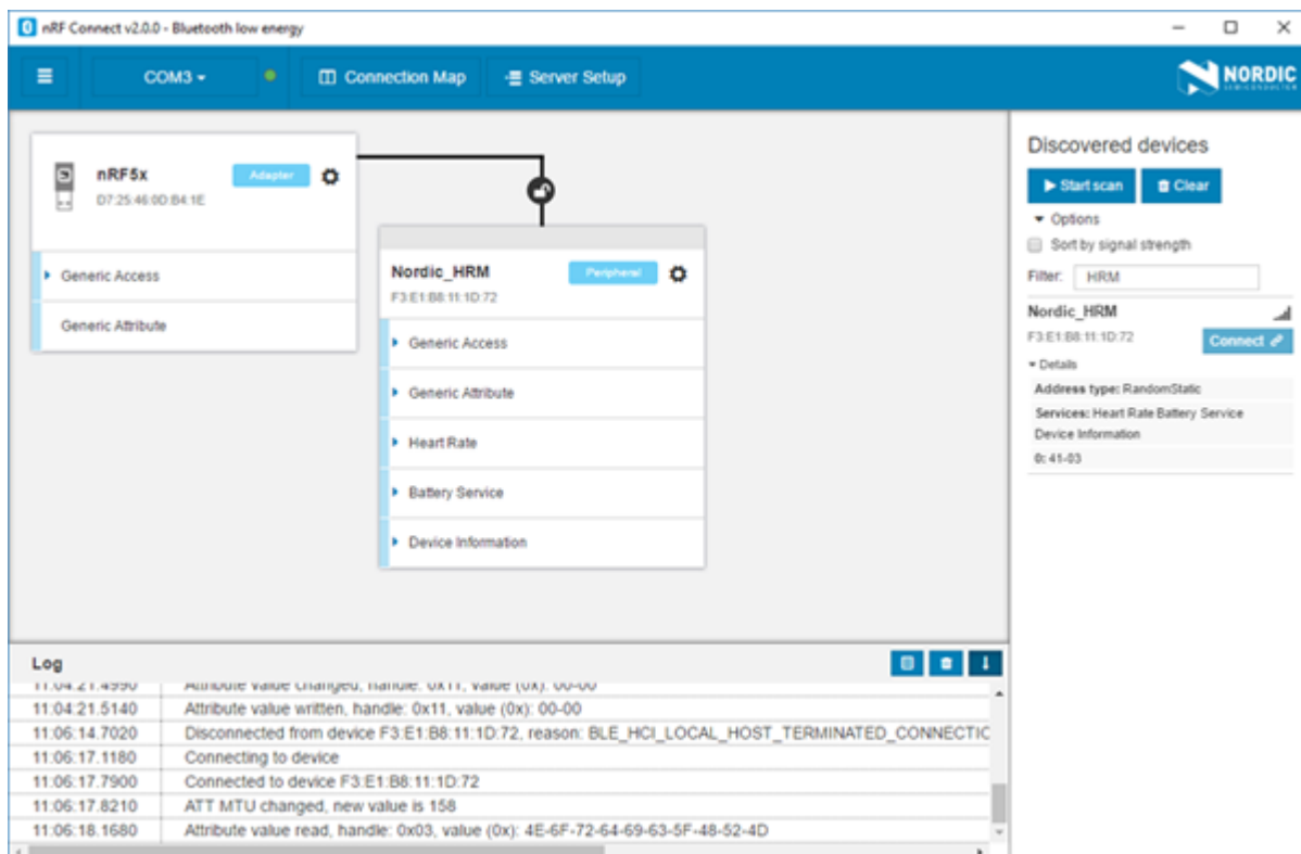
Figure 3: Discovered services
