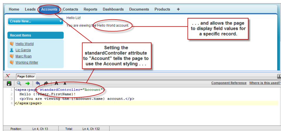
Figure 5: Displaying Account Data in a Visualforce Page
