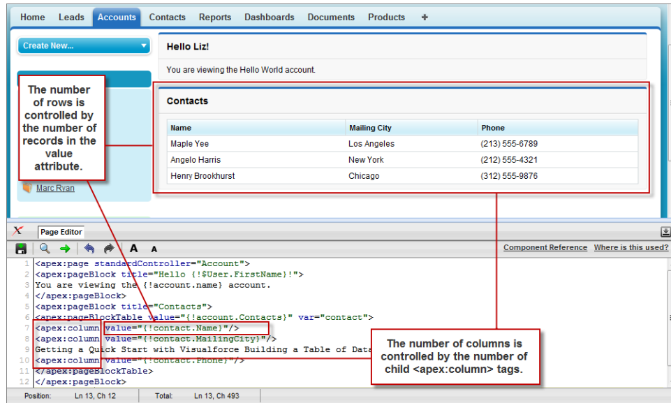
Figure 14: The <apex:pageBlockTable> Component
