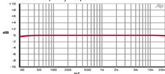
Pro48 Frequency Response
