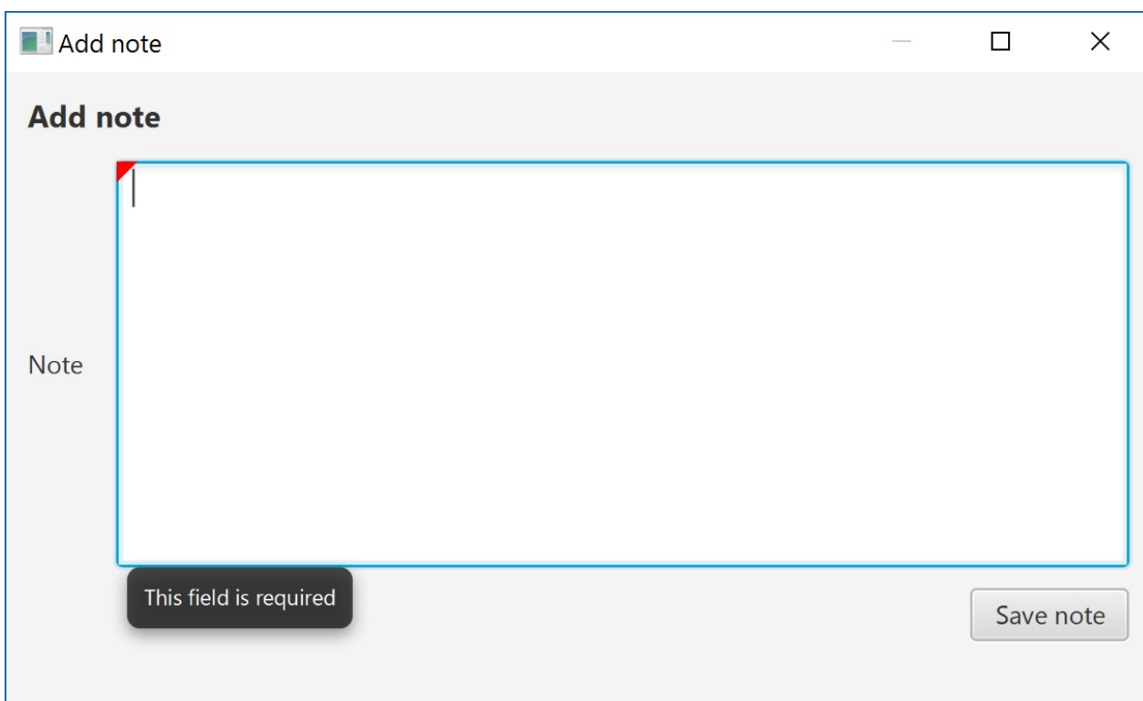
Figure 11.3 A dialog with an inline ViewModel context
