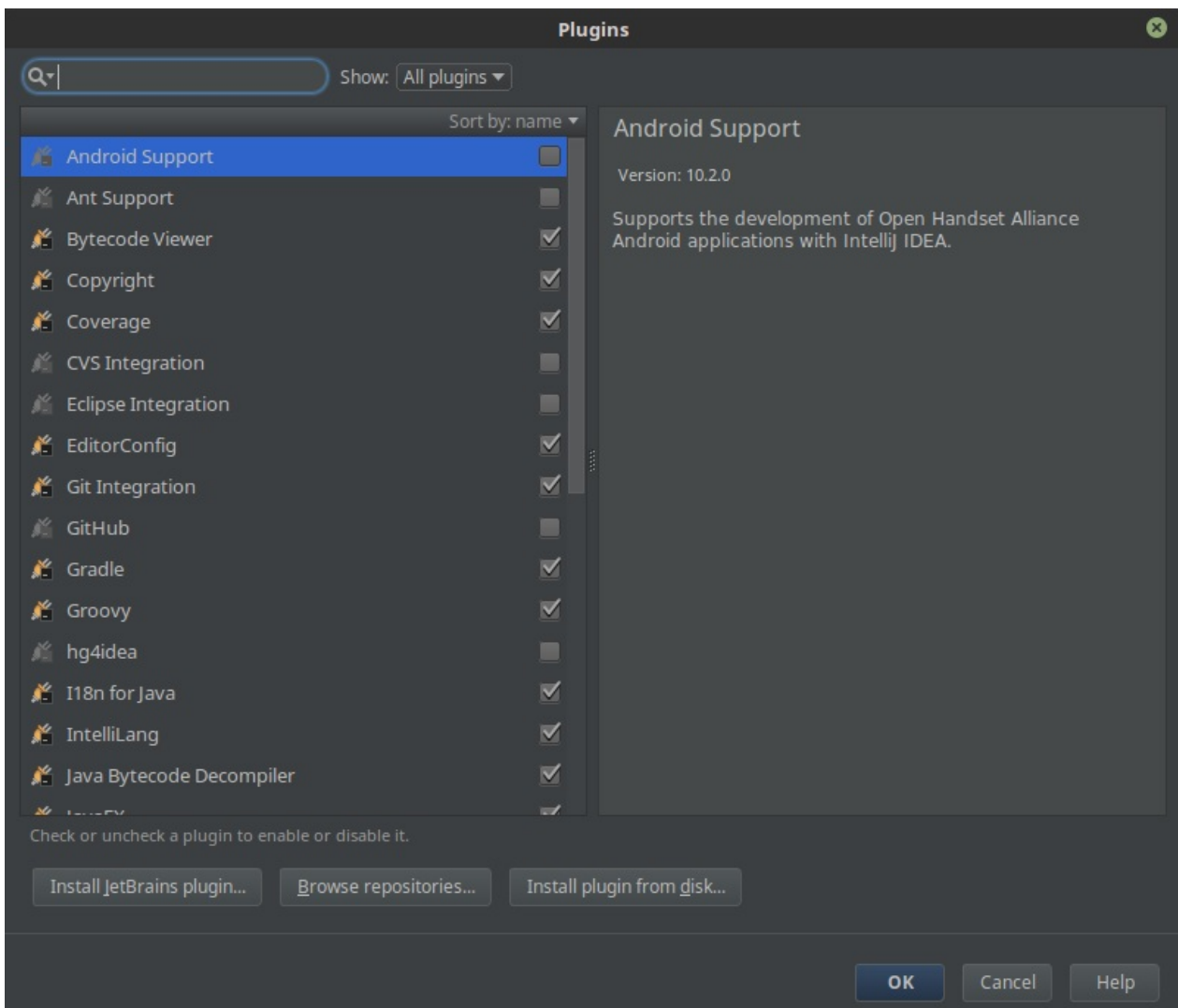
Figure 13.1 After bringing up the Plugins dialog, click Browse Repositories .
