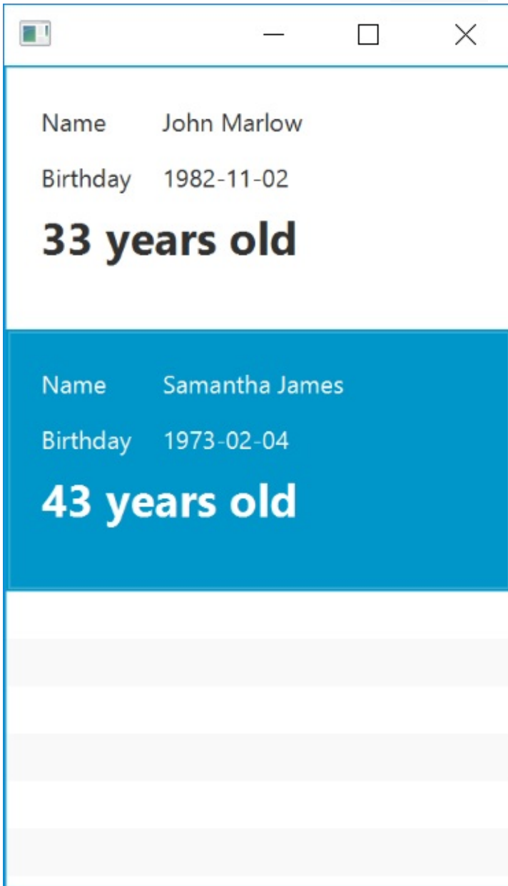
Figure 5.2 - A custom cell rendering for ListView
