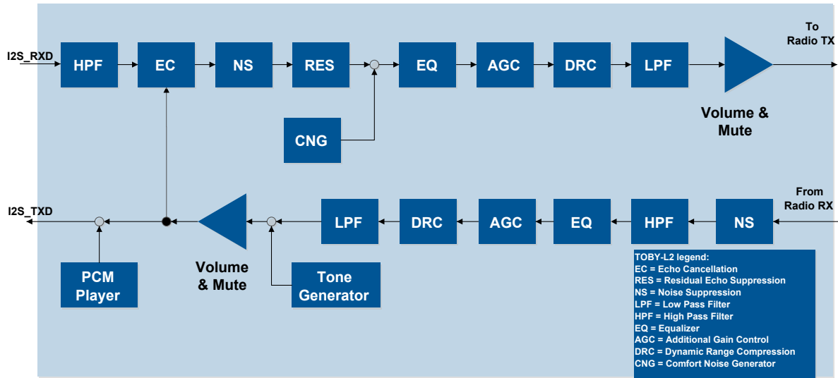
Figure 13: Audio paths
