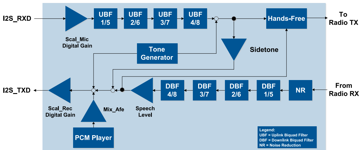
Figure 16: Audio paths
