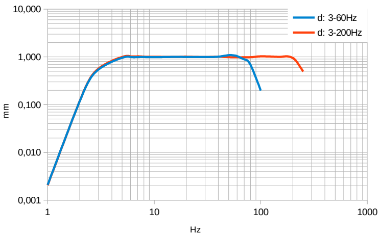
Figure 4: Frequency Response for vibration displacement
