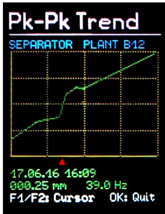
Figure 20: Trend Display
