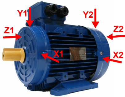
Figure 13: Measuring points on electric motors
