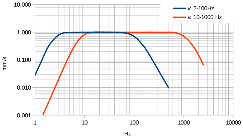
Figure 3: Frequency Response for vibration velocity
