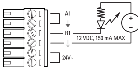
Figure 9. Relay Wiring
