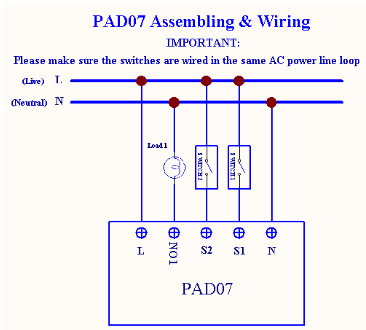
Fig 1. Assembling & Wiring
