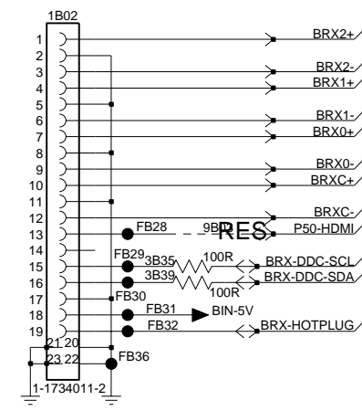
HDMI CONNECTOR 2
