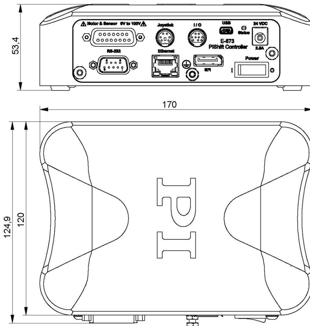
E-873.1A1, Abmessungen in mm
