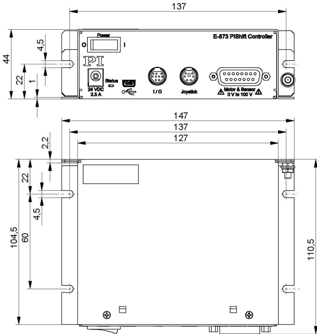
E-873.1AR, Abmessungen in mm
