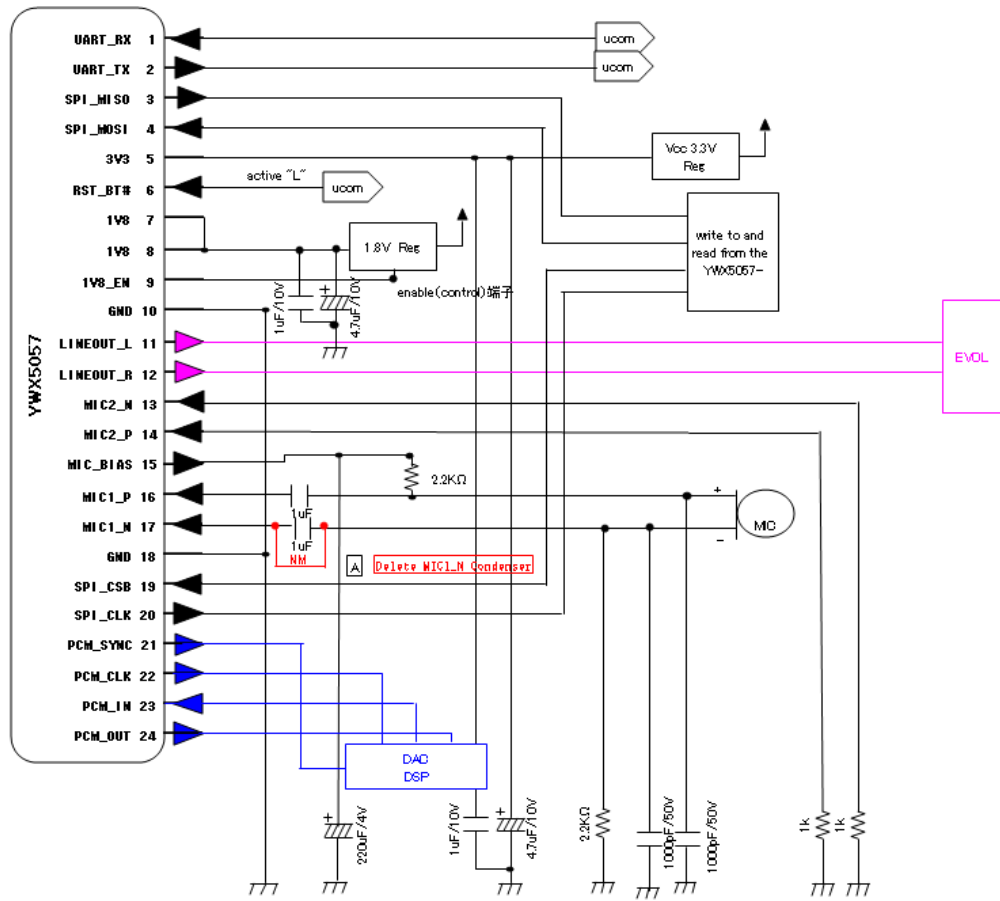
YWX5057 Pin-out diagram
