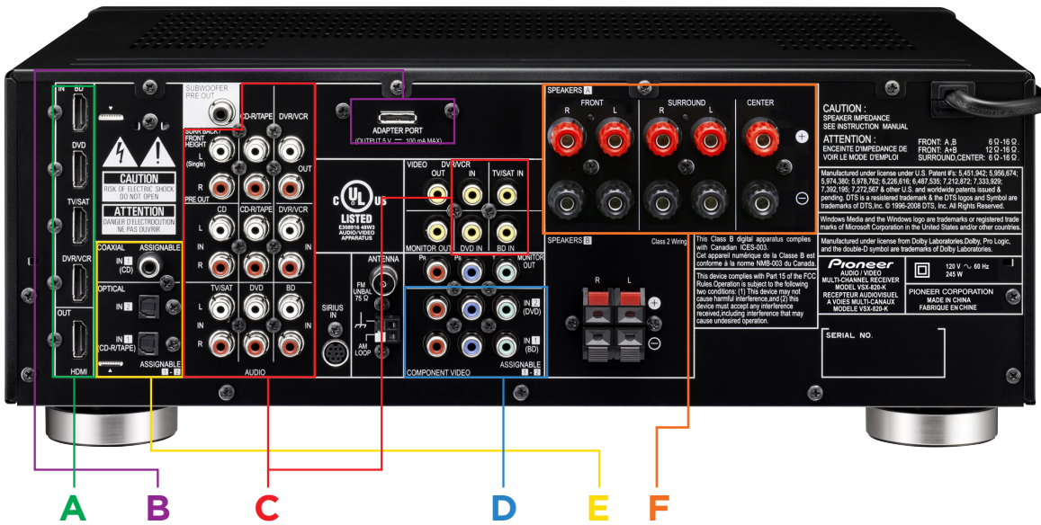
Rear Panel
