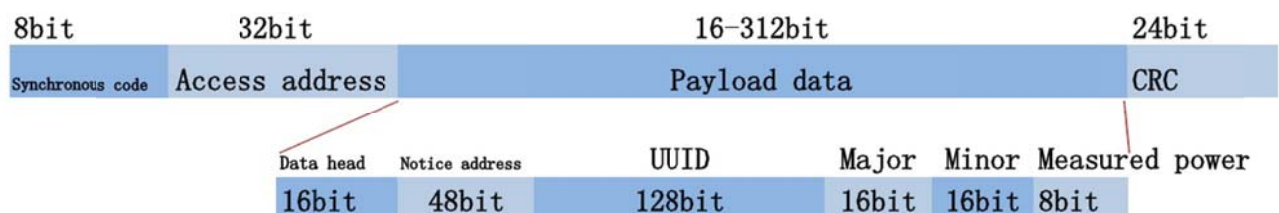
iBeacon Data frame structure
