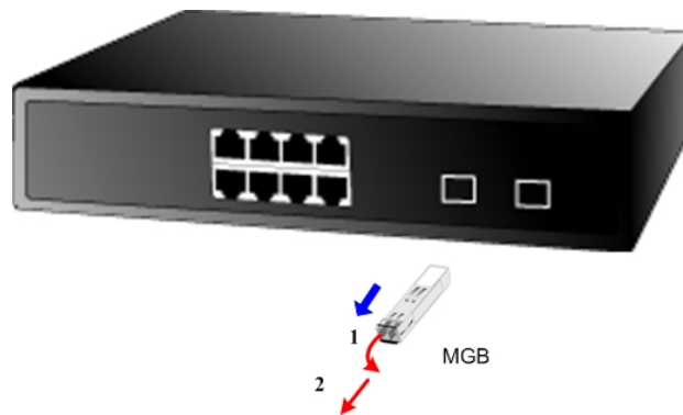
Figure 2-11 Pull out the SFP transceiver
