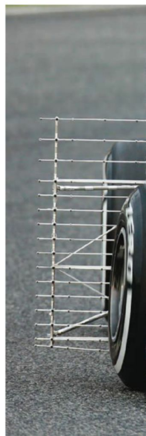
Early testing of the RB13 focused on shaking it down and evaluating aero correlation
