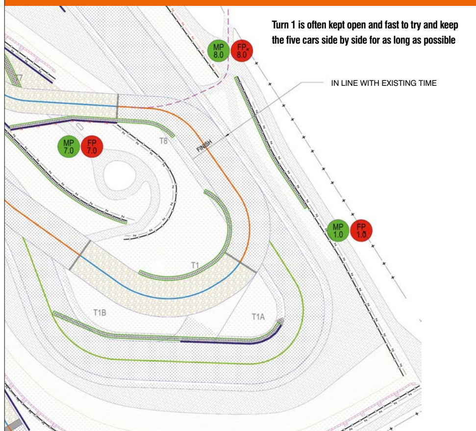
Figure 1: A typical track design drawing
