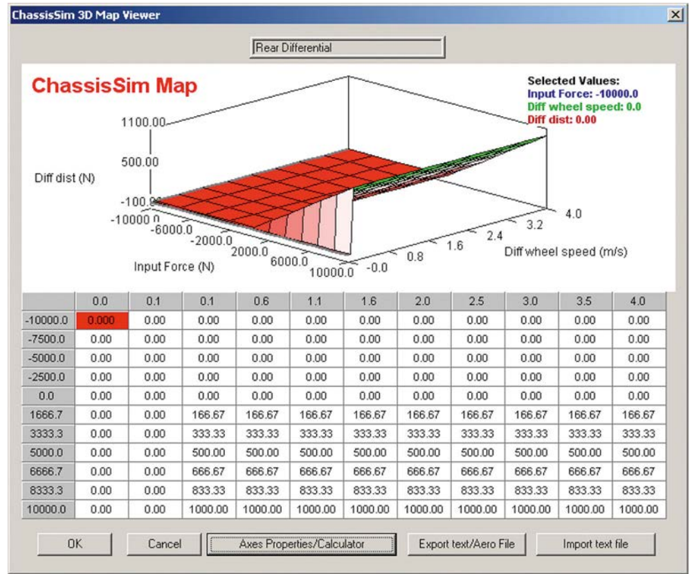
Figure 3: Differential dyno
