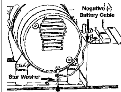
(-) Negative Battery Cable Connection
